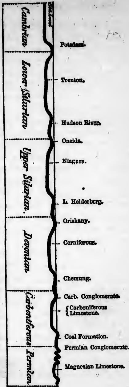
GEANTS SHOWING THE SUCCESSIVE ELEVATIONS AND DEPRESSIONS OF THE AMERICAN CONTINENT, IN THE SEVERAL CYCLES OF THE PALAEOZOIC ERA.
