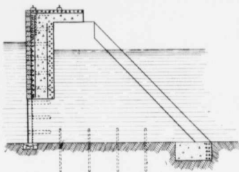
SECTION THROUGH INTAKE.
