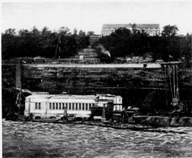
GENERATING AND DISTRIBUTING STATIONS DURING CONSTRUCTION.
