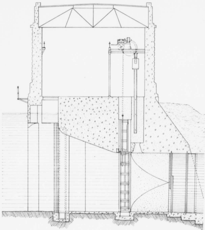
SECTION THROUGH GATE HOUSE.
