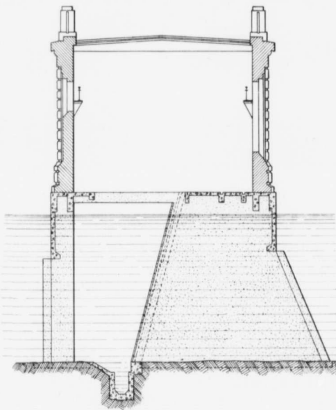
SECTION THROUGH SCREEN HOUSE.
