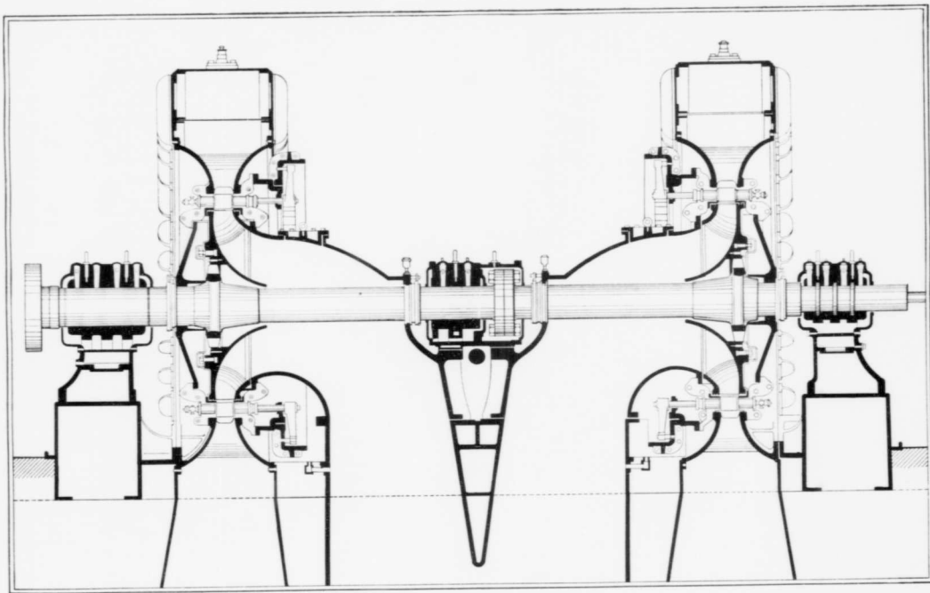
SECTIONAL DETAIL OF HORIZONTAL TURBINE.
