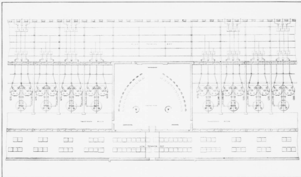
PLAN OF CENTRAL PORTION OF DISTRIBUTING STATION.
