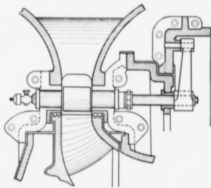
OPERATING MECHANISM OF TURBINE GATE.
