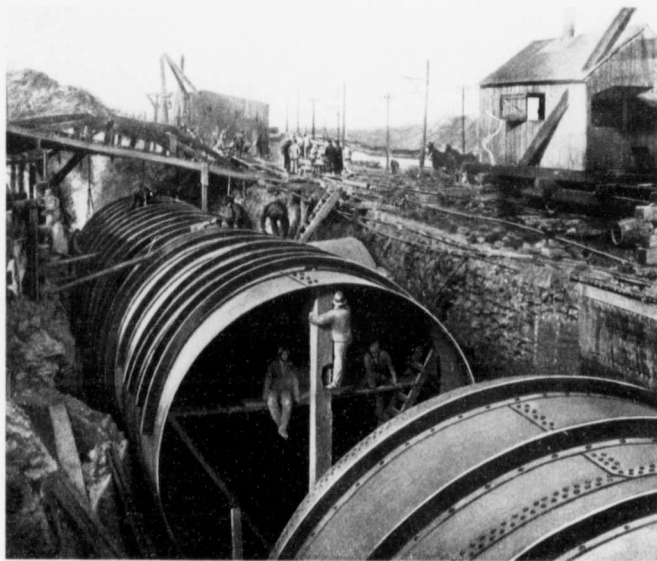
MAIN CONDUIT DURING CONSTRUCTION.
