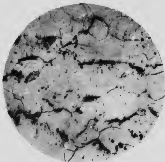
Microphotograph of serpentine, of randomly oriented olivine crystals.
