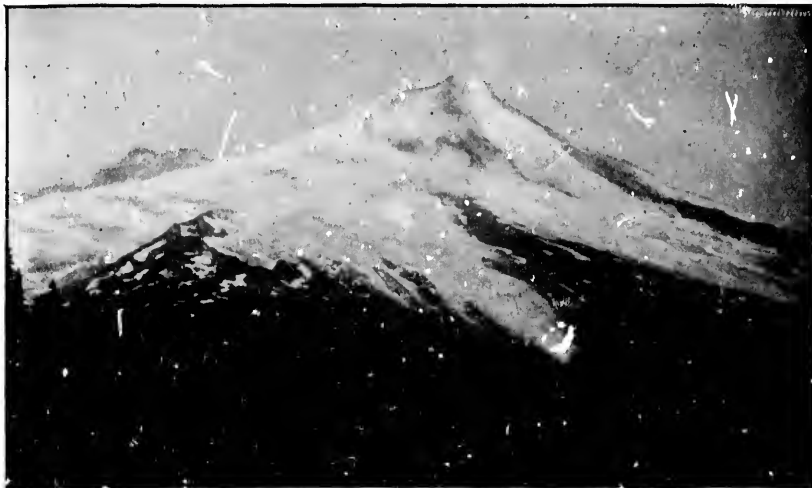
FIG. A.—SUMMIT OF MOUNT BAKER, WASHINGTON.
