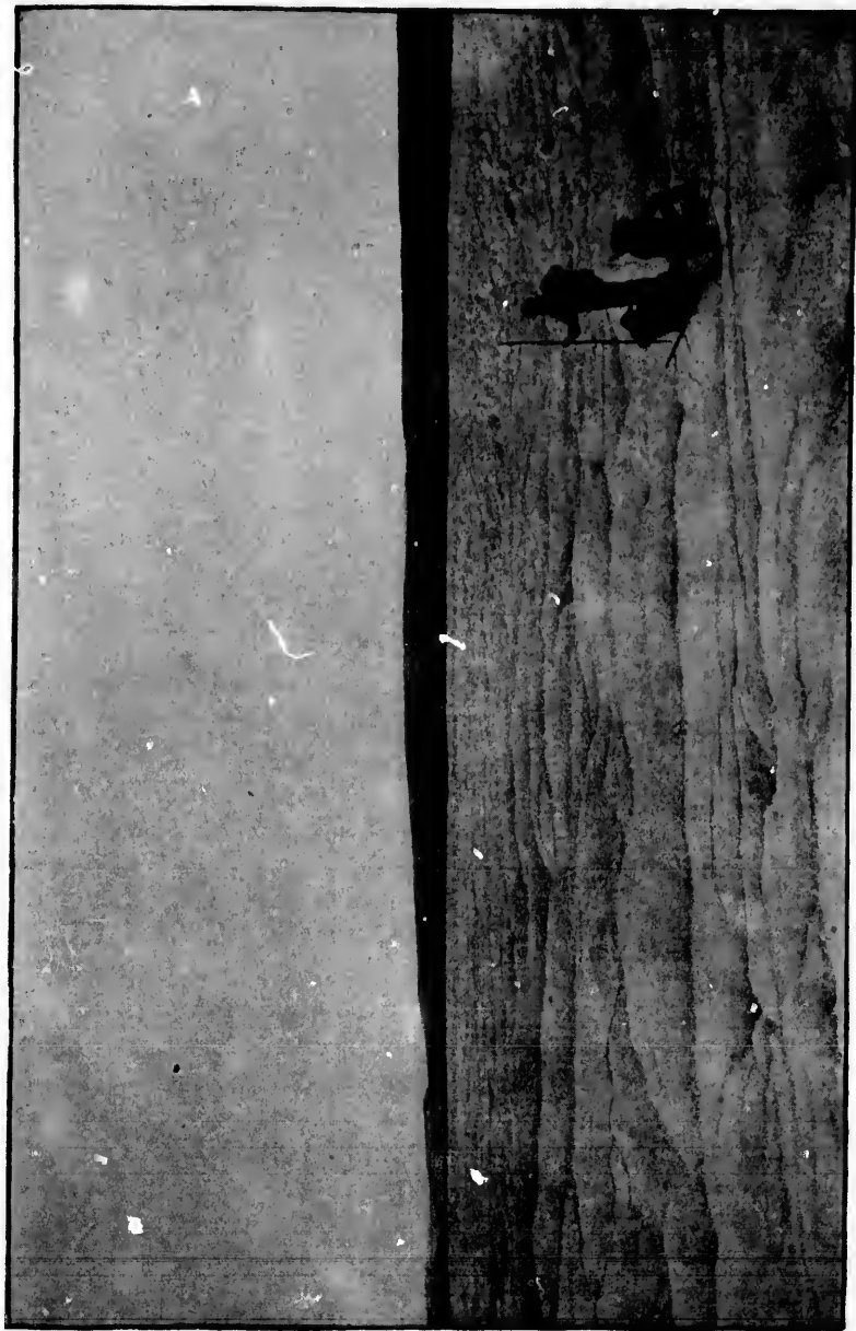
CENTRAL PORTION OF MALASPINA GLACIER, ALASKA.
