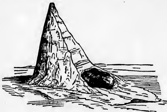
FIG. 4.—ICE PYRAMIDS, MOUNT LVELL GLACIER, CALIFORNIA.
