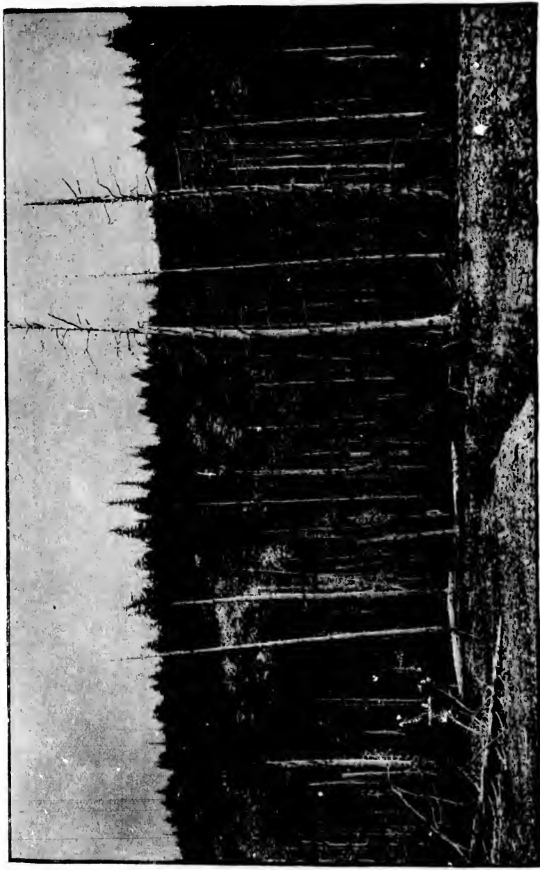
FRONT OF MALASPINA GLACIER, NEAR ICE BAY, ALASKA.
