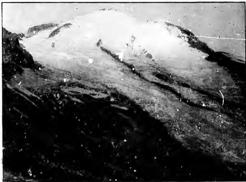
FIG. B. — SUMMIT OF MOUNT RAINIER, WASHINGTON.
