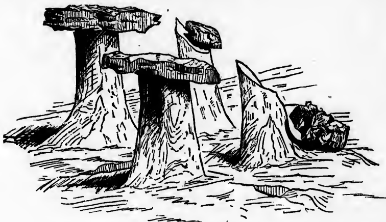
FIG. 3. — GLACIER TABLES, PARKER CREEK GLACIER, CALIFORNIA.
