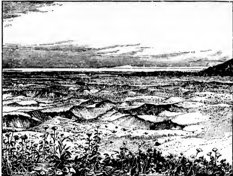
FIG. A.—MORaine-COVERED BORDER OF MALASPINA GLACIER, FROM BLOSSOM ISLAND.
