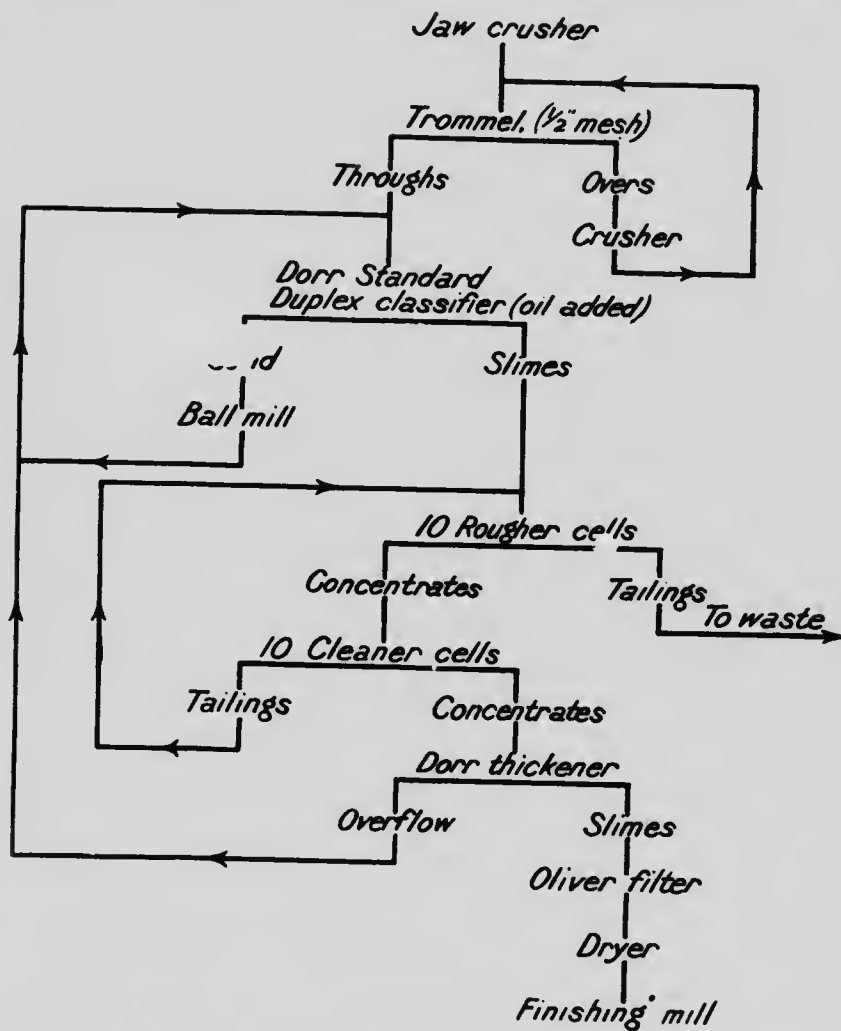
Fig. 30. Flow sheet of Minerals Separation oil flotation system, as installed in an Atabama mill.
