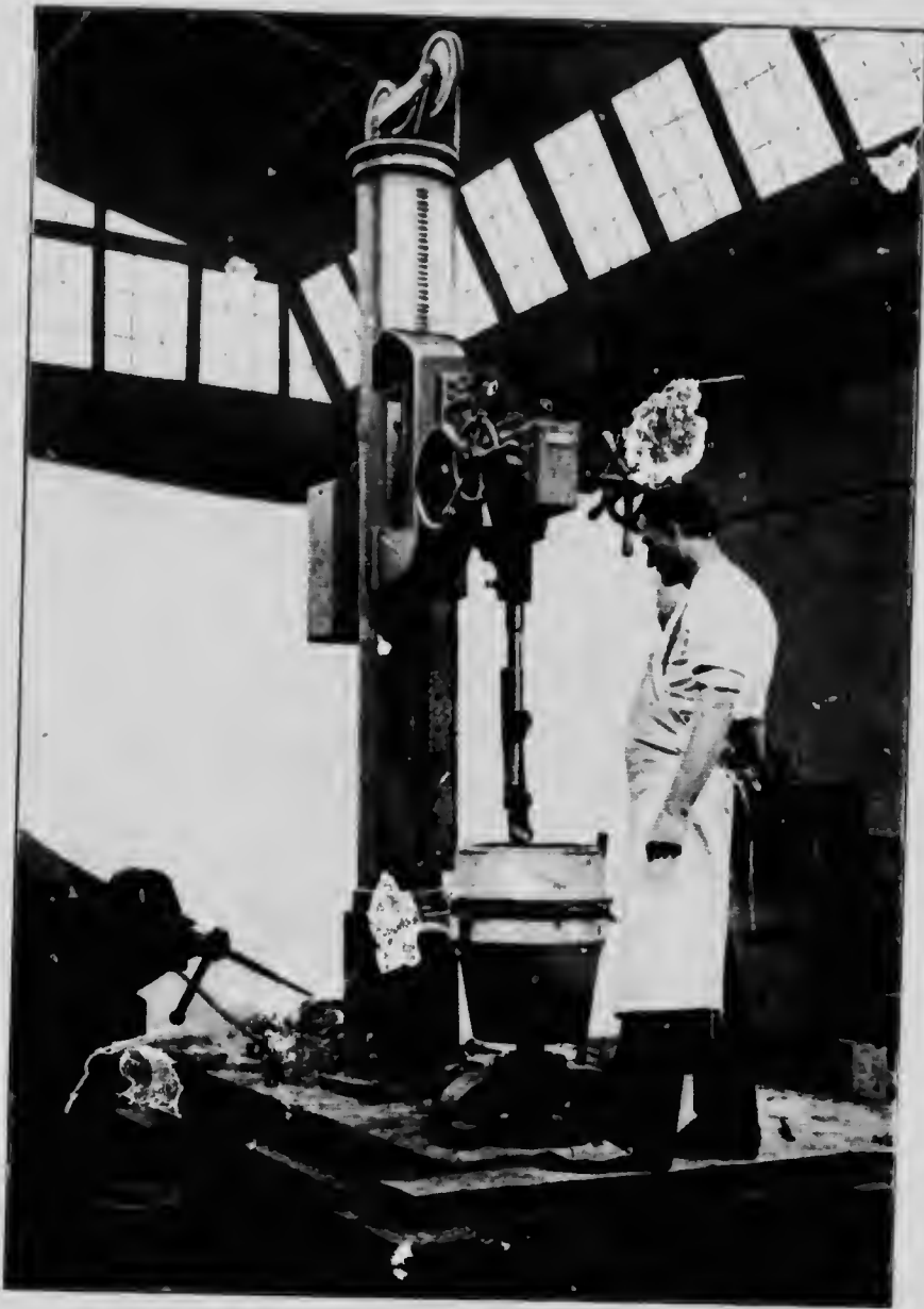
Pull-down and jigger used in making crucibles. (Crossley Machine Company, Trenton, N.J.) The illustration shows the profile or tool in position to be lowered into the mould by means of the right-hand wheel. The left-hand wheel controls the movement of the tool horizontally, in order to press the clay against the wall of the mould.
