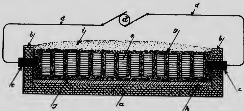
Fig. 40. Section through electric furnace arranged for graphitizing carbon electrodes of rectangular section. a , brick base; b , end walls; c , electrodes; d , connexions to source of energy d' ; e , electrode charge; g , layer of powdered coal or coke; h , refractory lining; i , covering of sand and powdered coke.
