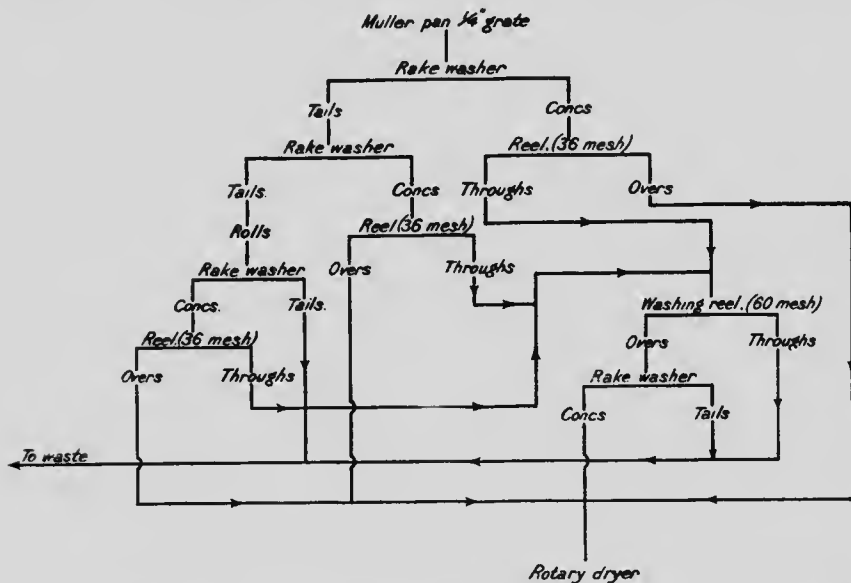
Fig. 24. Flow sheet of wet concentration system, using rake washers, in a Pennsylvania mill. This mill has a capacity of 100 tons of ore per 24 hours, requires 60 H.P. for operation, and three men to a shift.
