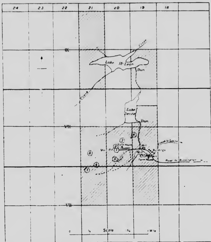
Fig. 8. Plan of workings, etc., at Walker mine, township of Buckingham, Quec. Openings 1-5 are in flake graphite; 6-8 in phosbago.
