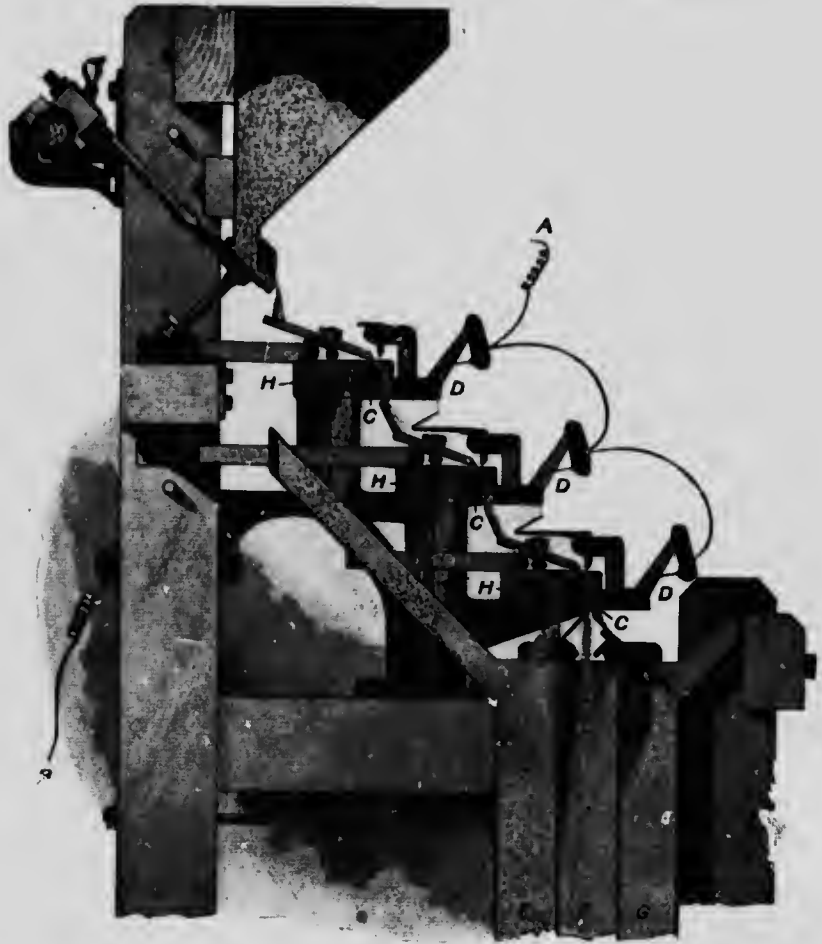
Details of Sutton, Steele and Steele dielectric separator. A connexion to generator, B connexion to ground, C revolving electrode, D needle electrodes, E tailings, F middlings, G concentrates, H roller to remove particles adhering to electrode C.
