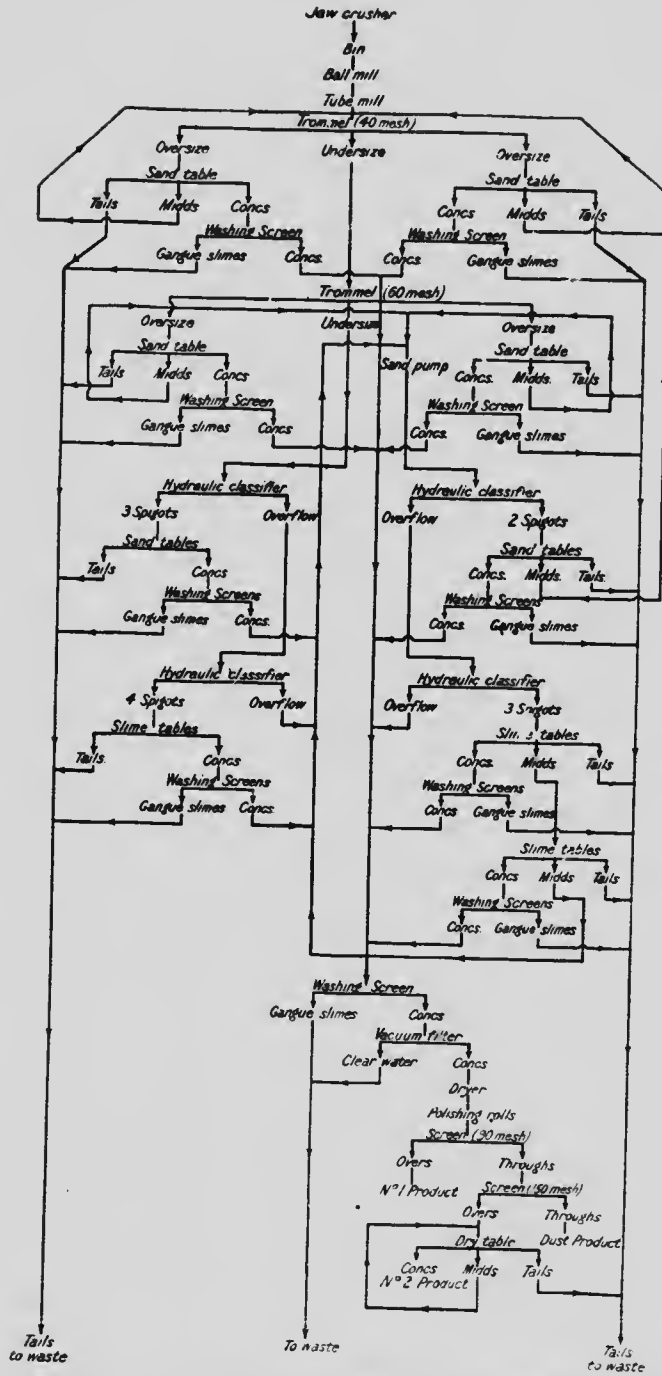
Fig. 27. Flow sheet of wet concentration system, using Ferraris tables, as installed in a Quebec mill.
