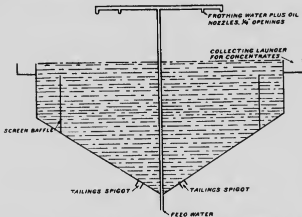
Fig. 32. Section through Simplex washer: not drawn to scale. Washer is elliptical, and measures about 6 feet by 3½ feet. (United States Bureau of Mines.)
