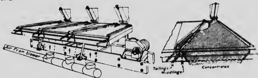
Fig. 13. Sutton, Steele and Steele three-section jig.
