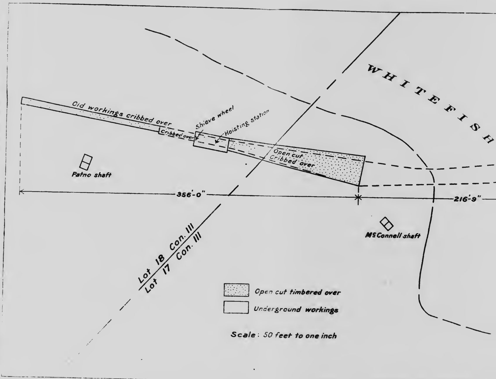
Fig. 4. Plan of workings, Black Donald
