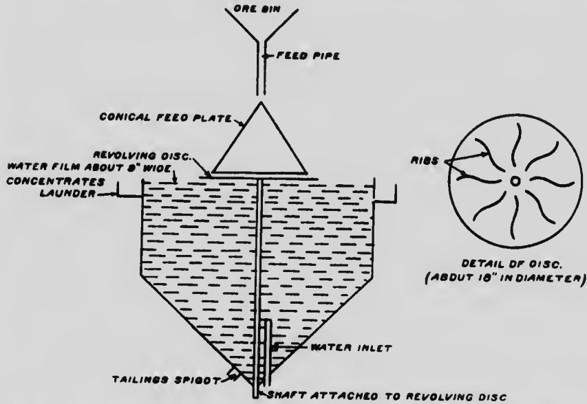
Fig. 35. Section through Colmer washer (not drawn to scale). The washer is about 3 feet in diameter. (United States Bureau of Mines.)
