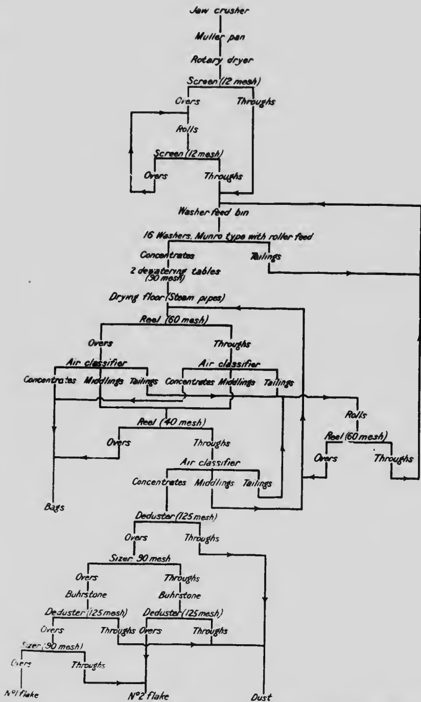
Fig. 37. Flow sheet of surface tension concentration installation, using Munro washers, in an Alabama mill.
