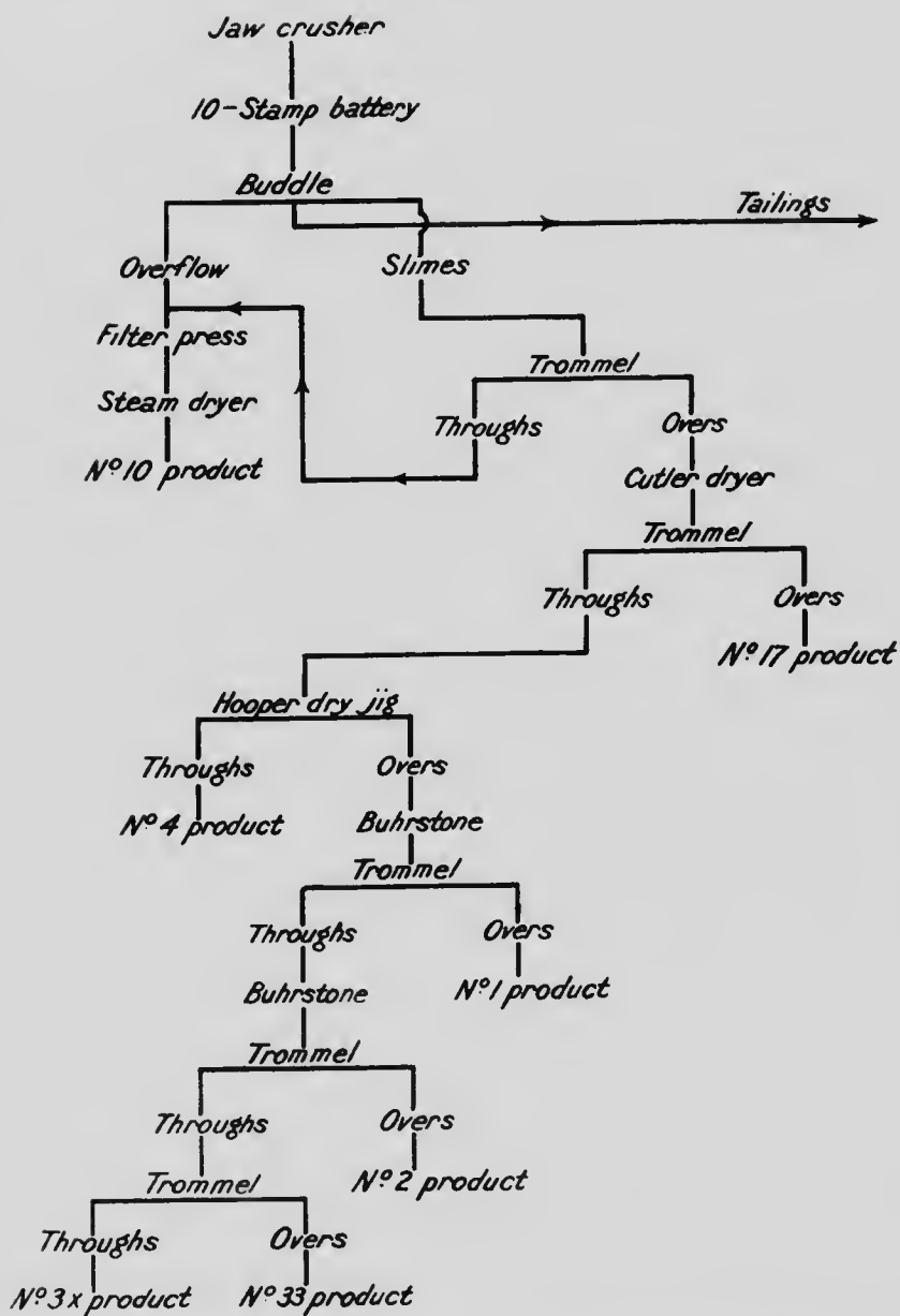
Fig. 22. Flow sheet of combined wet and dry concentrating system, as installed in an Ontario mill.
