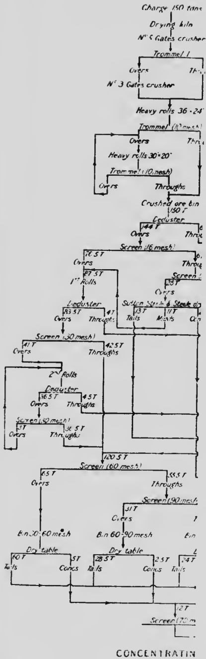
Fig. 18. Flow sheet of dry concentration of dry concentration of
