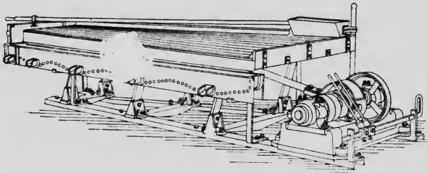
Fig. 25. Ferraris type of wet table.
