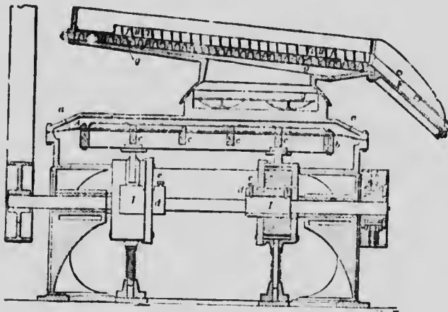
Fig. 12. Section through Hooper pneumatic concentrator.
