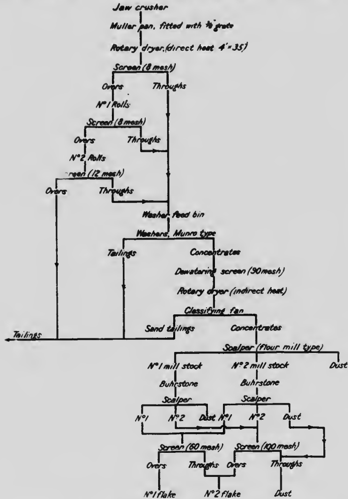
Fig. 36. Flow sheet of surface tension concentration installation, using Munro washers, in an Alabama mill.
