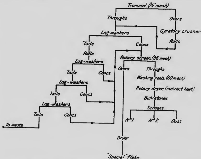
Fig. 23. Flow sheet of mill employing log-washer concentration, Byers, Pennsylvania. The ore is very decomposed, and comes to the mill in the form of gravel.
