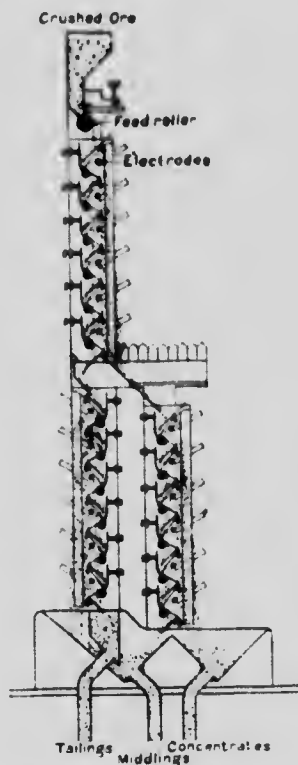
Fig 20. Section through Huff electrostatic separator.
