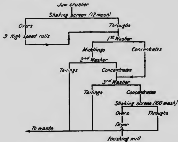
Fig. 31. Flow sheet showing Simplex oil flotation system, as installed in an Alabama graphite mill.
