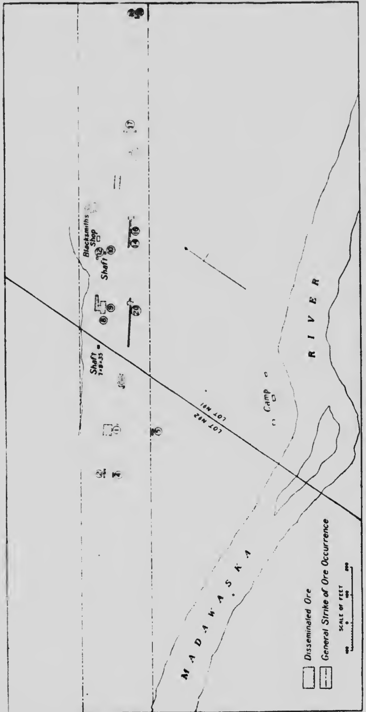
Fig. 5. Surface plan of graphite showings on lots 1 and 2, concession 11, township of Lyndoch, Ont.
