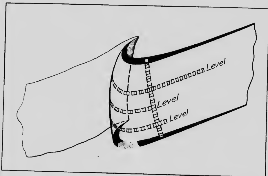
Fig. 2. Diagram showing approximate form of graphite ore-body on crest of pitching anticline, lots 21 and 22, concession VI, North Elmsley township, Ontario.
