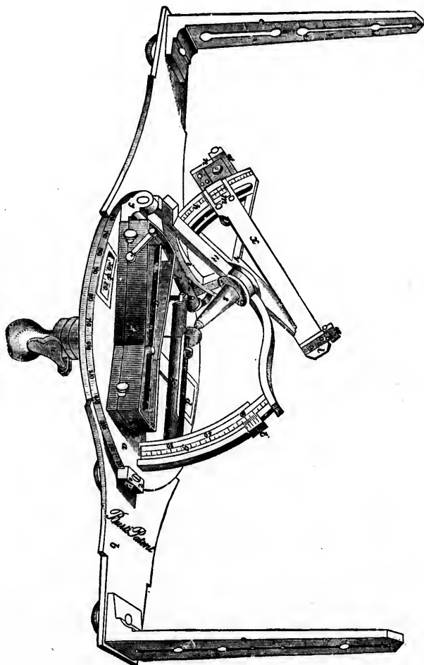
HURT'S SOLAR COMPASS.
