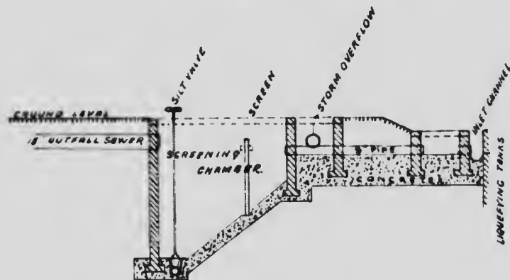
FIG 6. SCREENING CHAMBER
