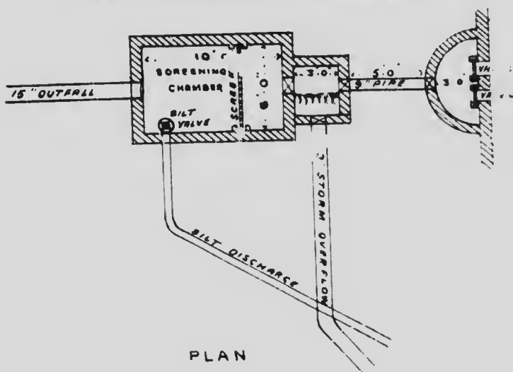
FIG. 5. SCREENING CHAMBER.
