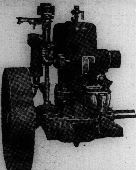
5 H.P. Imperial Fishermen's Engine.
