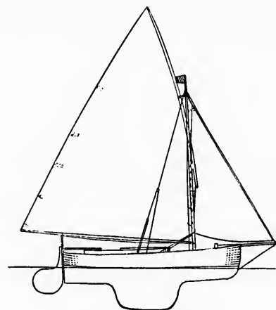
HUMMING BIRD.—FIGURE 131.
