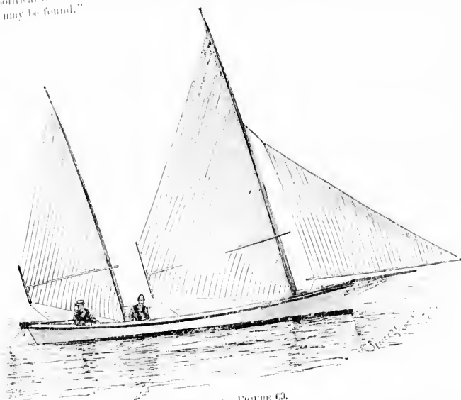
CHESAPEAKE.—FIGURE 60.
