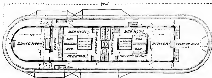
PLAN OF THE "CAJMAN."
