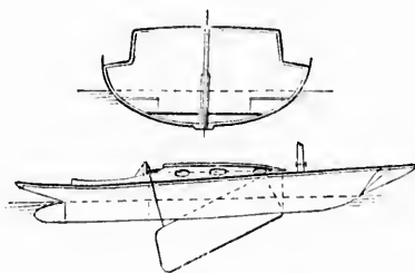
ROCKET.—FIGURE 122.
