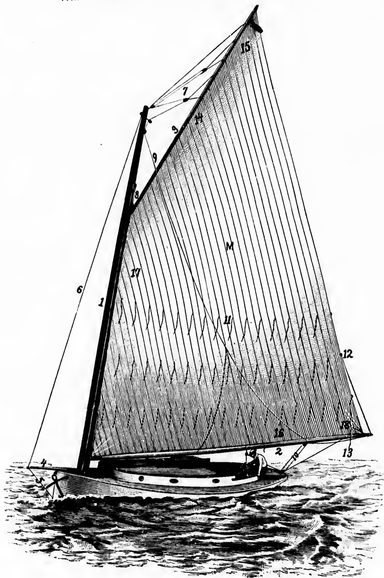
THE CAT BOAT.—FIGURE 189.
