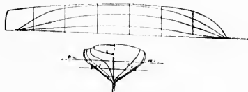
CYGNET.—FIGURE 106.
