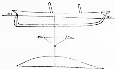
AMERICA.—FIGURE 107.
