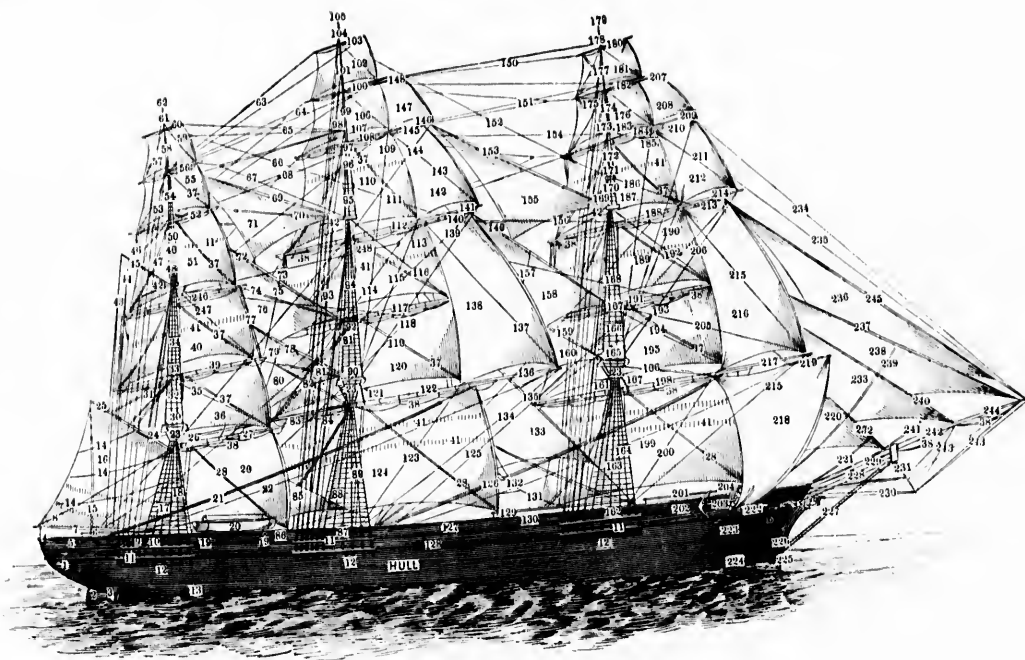
FULL RIGGED SHIP.—FIGURE 197.
