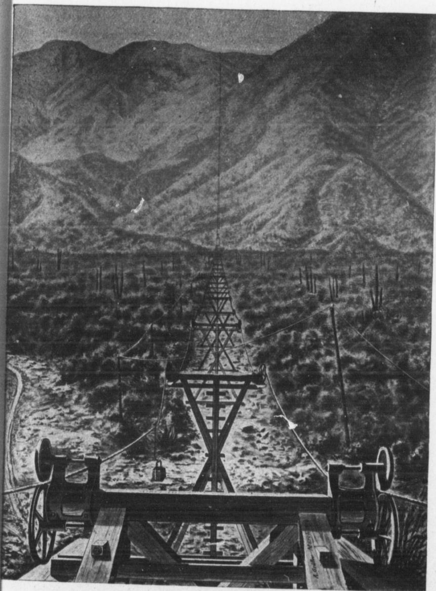
SINGLE ROPE CABLEWAY BUILT BY CALIFORNIA WIRE WORKS.
