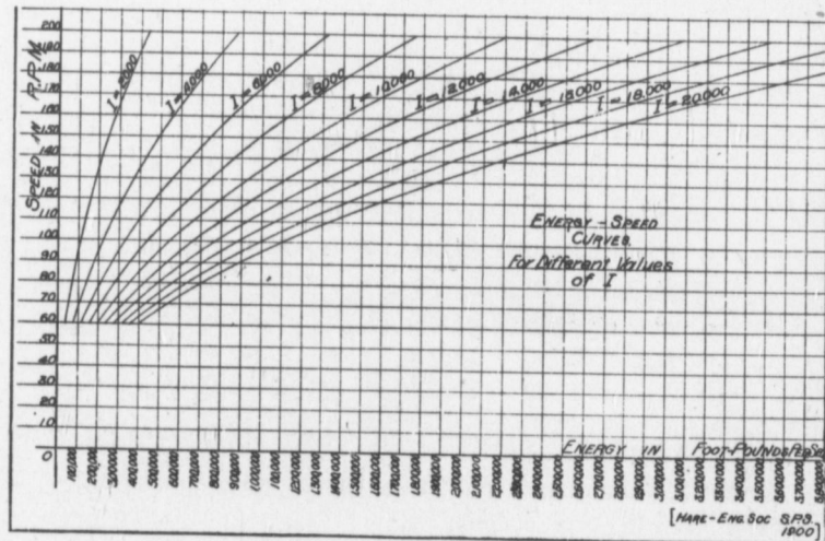
FIG. 2.—KINETIC ENERGY—SPEED CURVES, FOR FLYWHEELS.
