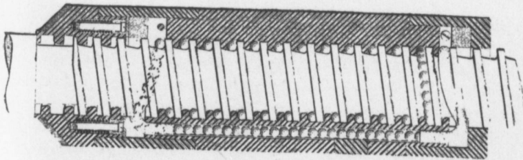
FIG. 9.—SECTION OF SCREW AND SLIDING NUT.
