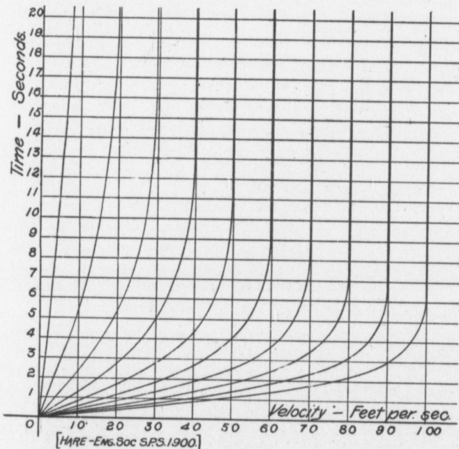
FIG. 1.—TIME—VELOCITY CURVES, FOR SUPPLY PIPES.
