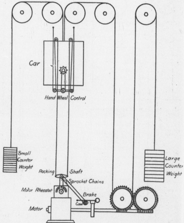
FIG. 7.—DIRECT CONNECTED ELECTRIC ELEVATOR.
