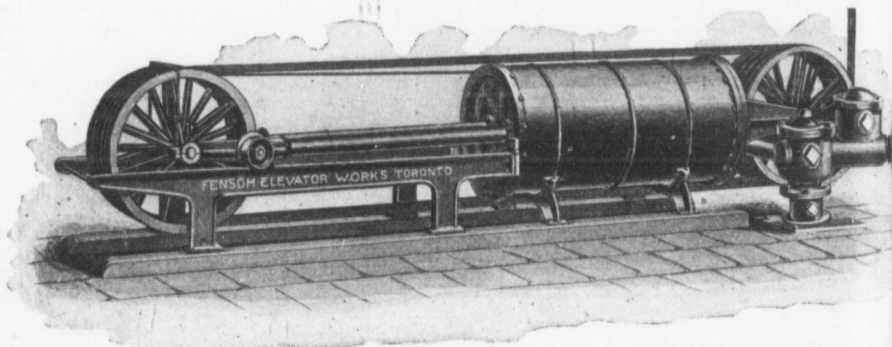
FIG. 4.—HORIZONTAL HYDRAULIC ELEVATOR.
