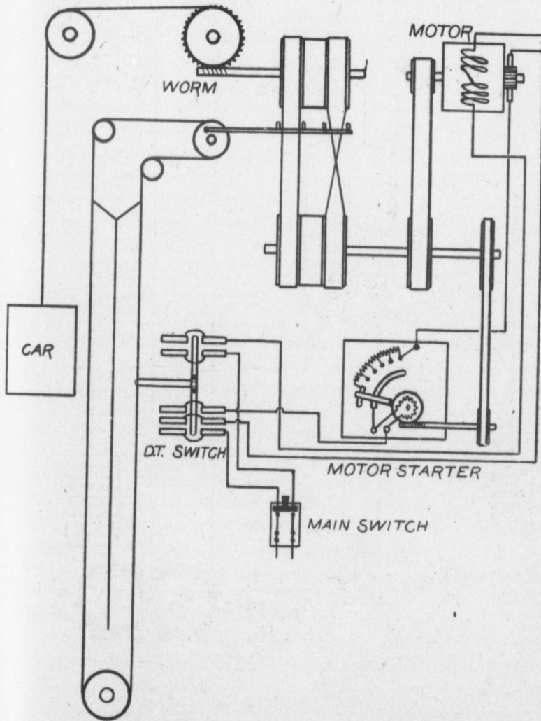
FIG. 6.—BELT DRIVEN ELECTRIC ELEVATOR.
