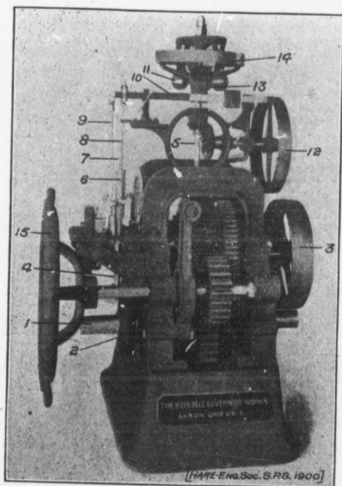
FIG. 5.—"REPLOGLÉ" WATER WHEEL GOVERNOR.
