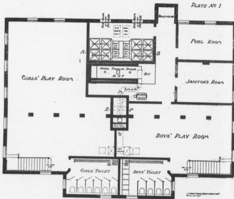
PLAN OF FOUR ROOM SCHOOL DESIGNED TO SHOW METHOD OF VENTILATION See Description
