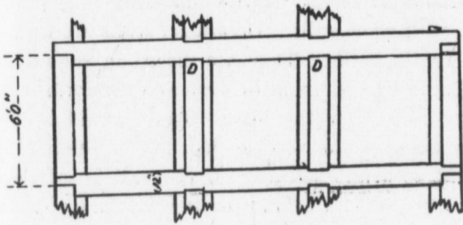
Fig 1 Elevation
