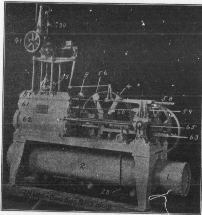
FIG. 3.—"Lombard" WATER WHEEL GOVERNOR (Side view).
