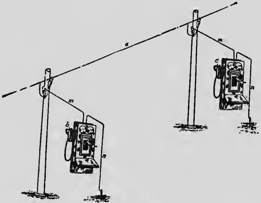
Fig. 1.—Diagram Showing Connections of the Grounded System.
