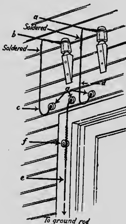
Fig. 41—The Drop Wires are Fastened to the House as Here Shown.
