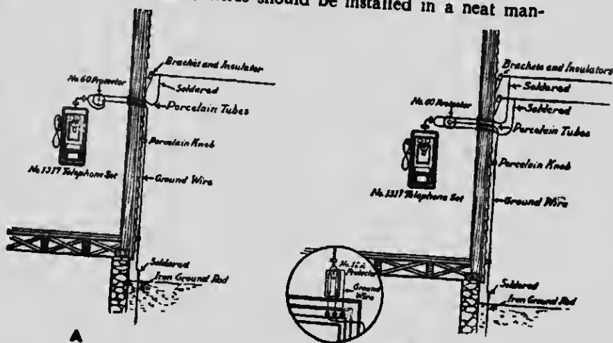
A Fig. 43—Methods of Wiring a Telephone Set and Protector: A on a Grounded System; B on a Metallic System.
