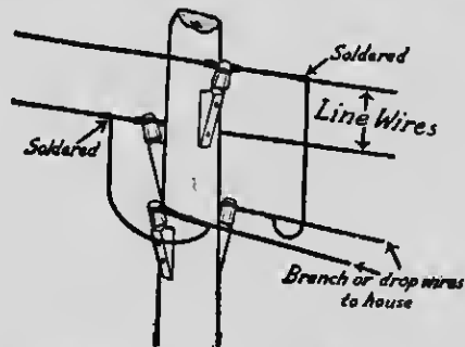
Fig. 40—Method of Attaching Branch or Drop Wires to the Pole.
