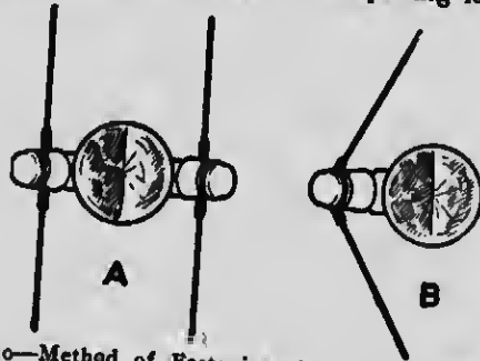
Fig. 30—Method of Fastening the Line Wires to the Insulators—A on Straight Lines; B at Curves.
