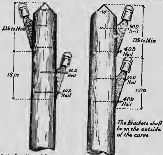
Fig. 6—Location of Brackets on Pole at Curves.
