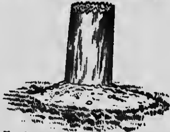
Fig. 18—Earth Should be Slightly Banked Around the Pole as Here Shown.
