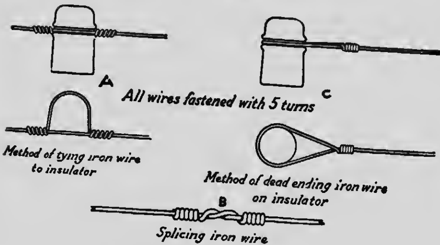
Fig. 31—Details of Tying, Splicing and Dead Ending Iron Line Wire.
