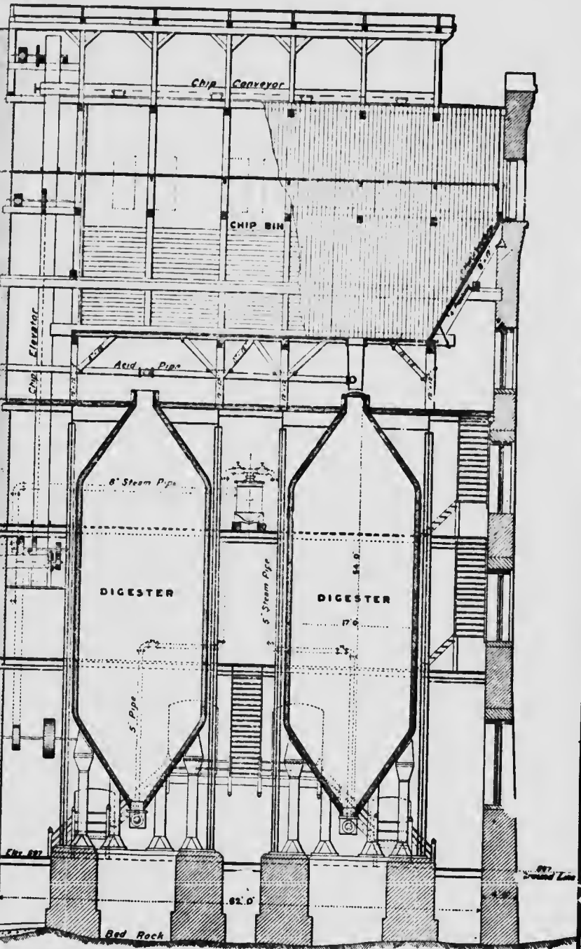
DIGESTER HOUSE.
