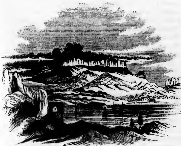
BASALTIC ROCKS.
