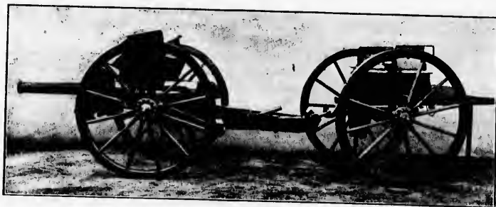
12½-POUNDER QUICK-FIRING FIELD-GUN—CITY OF LONDON FIELD BATTERY. By permission of Messrs. Vickers, Sons & Maxim, and the publishers of the Engineer .)
