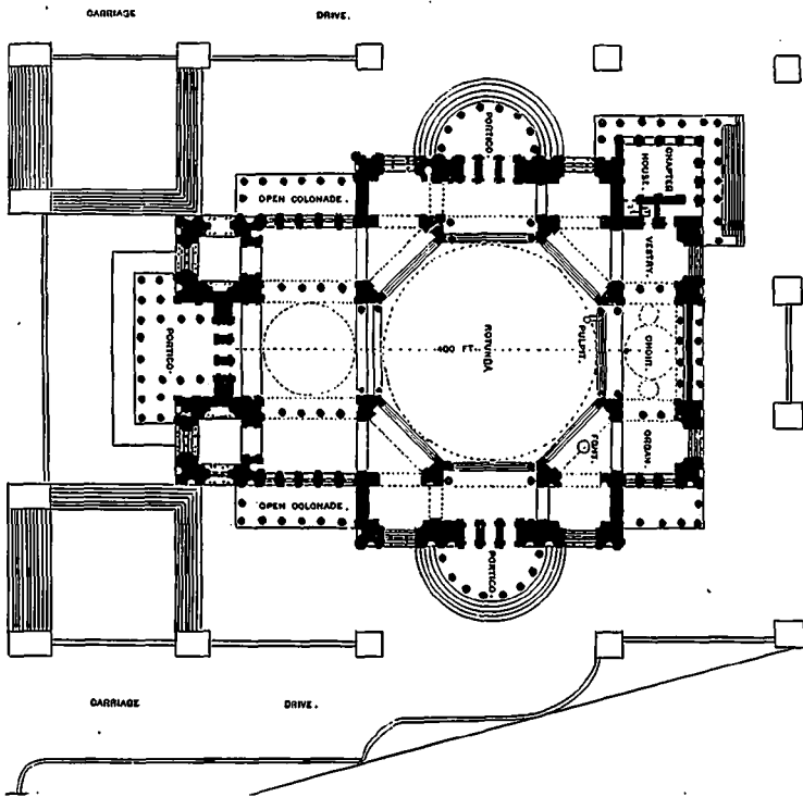
PLAN FOR CATHEDRAL OF ST. JOHN THE DIVINE, NEW YORK.
