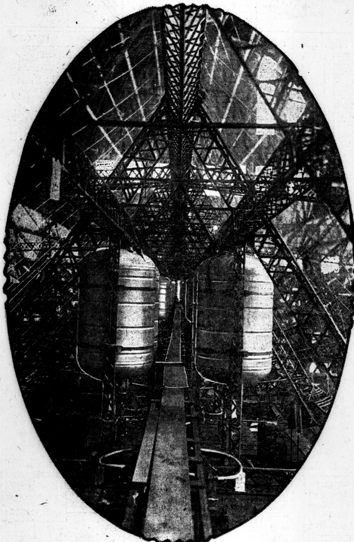
A view through the keel of the new dirigible ZR-1 showing some of the 48 gasoline tanks which hold 113 gallons each. They are built so that 16 can be slipped from the ship to lighten the weight in case of necessity.
