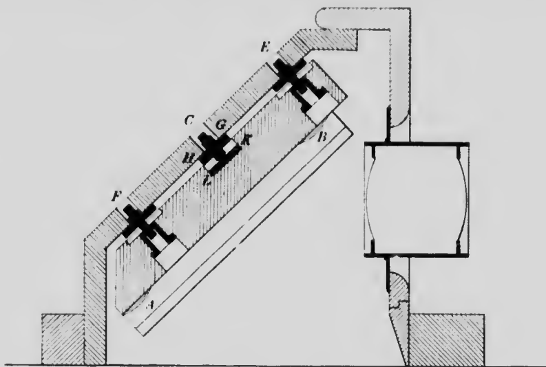
FIG. 20 b . Mirror box.
