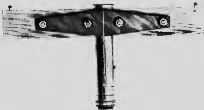
FIG. 12—Optical Square.
