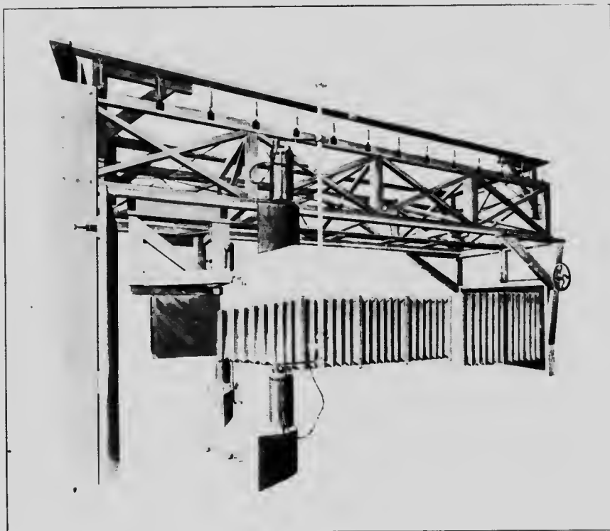
Fig. 2 Camera fitted with long bellows for enlarging.
