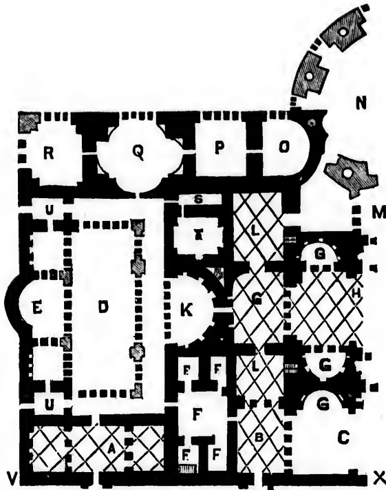
HALF OF THE PLAN OF THE BATHS OF CARACALLA. THE SIDE IN THE LINE V X FACING THE VIA NOVO; THE OPPOSITE SIDE OPENING UPON THE GARDENS.
