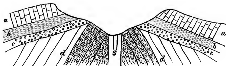
SECTION OF TUSCAN SPRINGS, CALIFORNIA.
