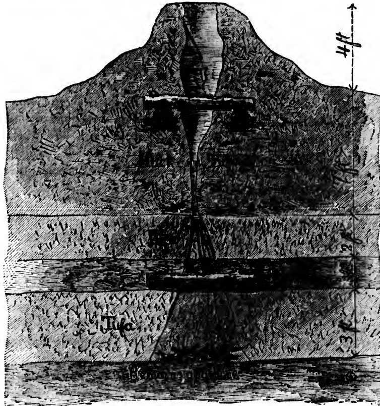
GEOLOGICAL SECTION AT SARATOGA SPRINGS.
