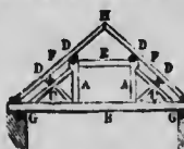
Queen-post roof.
