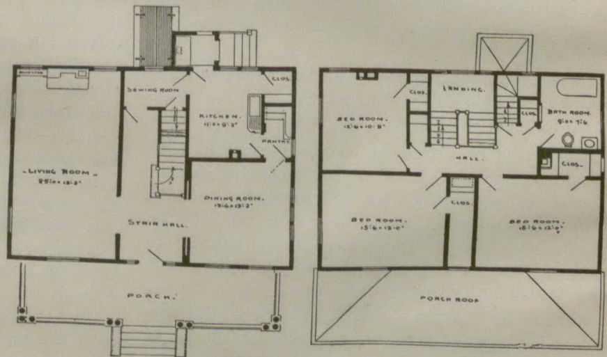
FIRST FLOOR SECOND FLOOR DESIGN FOR A MODERATE COST HOUSE.
