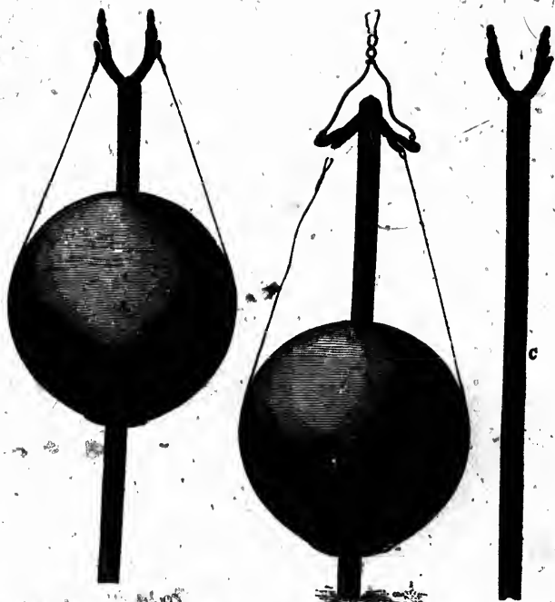
BROOKER'S DEEP SEA SOUNDING APPARATUS.
