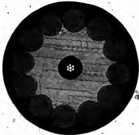
SHORE END—EXACT SIZE.
