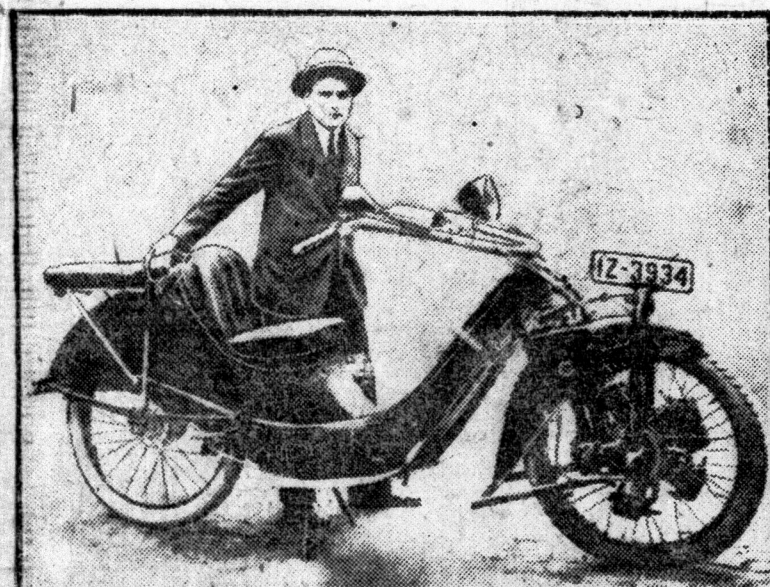
A wierd German motorcycle with all its engine mechanism in its front wheel. To start it, you hoist it on its stand, put on a pair of gloves and draw the wheel around as quickly as possible till one of the five cylinders fires.
