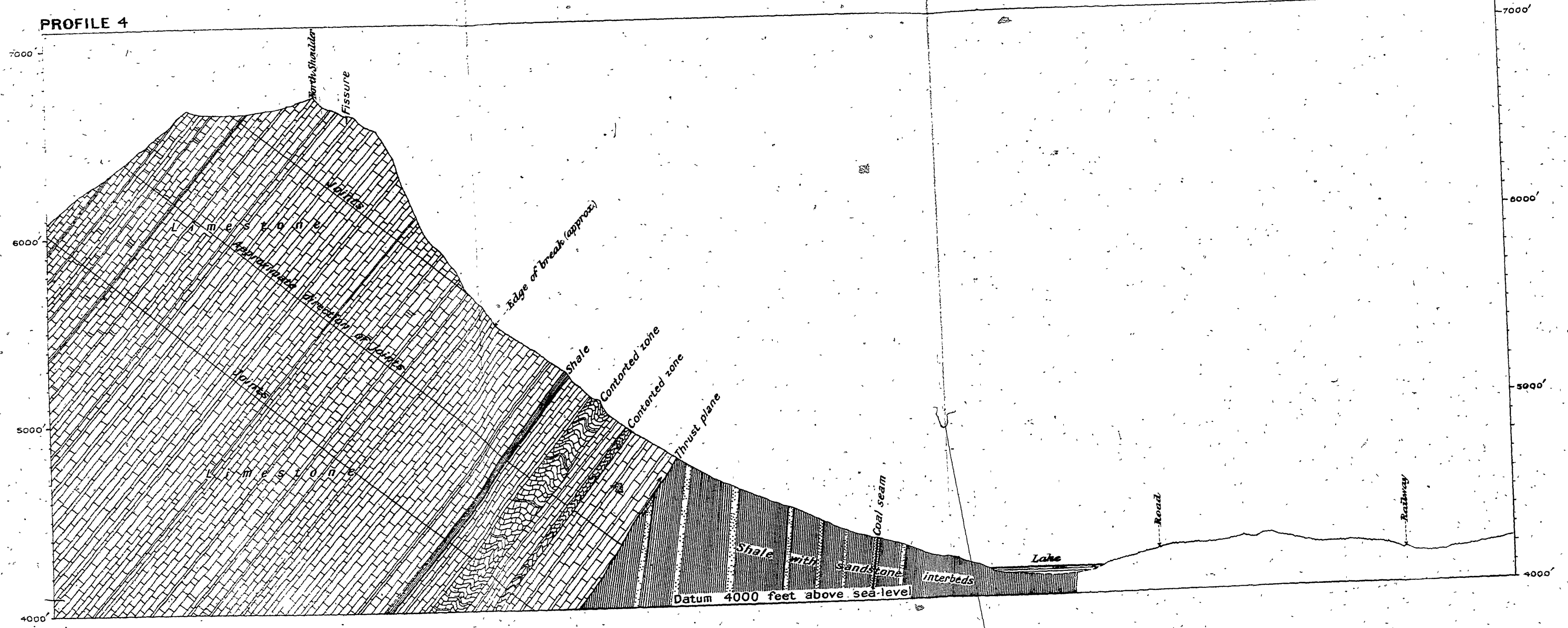
DIAGRAMMATIC SECTION ALONG PROFILE showing geological structure of TURTLE MOUNTAIN
