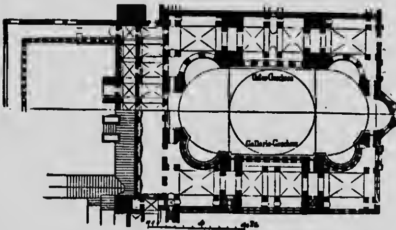
GROUND-PLAN OF THE CHURCH OF S. SOPHIA
