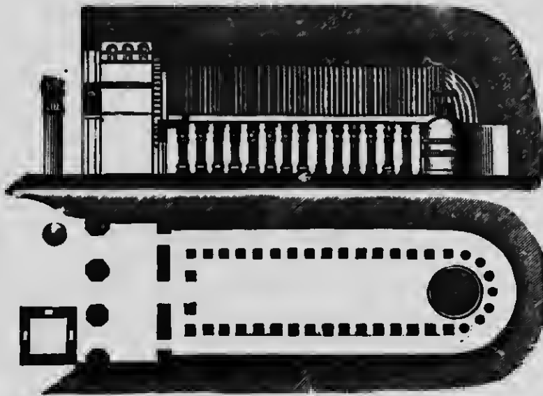
CAVE OF KARLI. SECTION AND GROUND-PLAN
