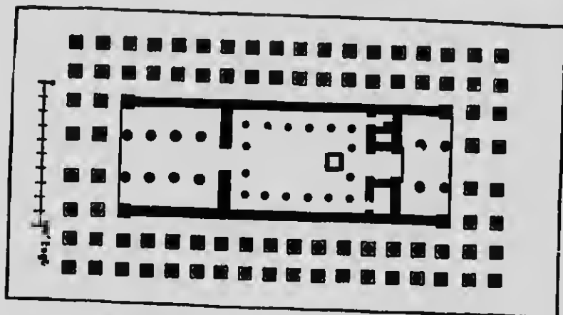
GROUND-PLAN OF DOUBLE PERIPTERAL
