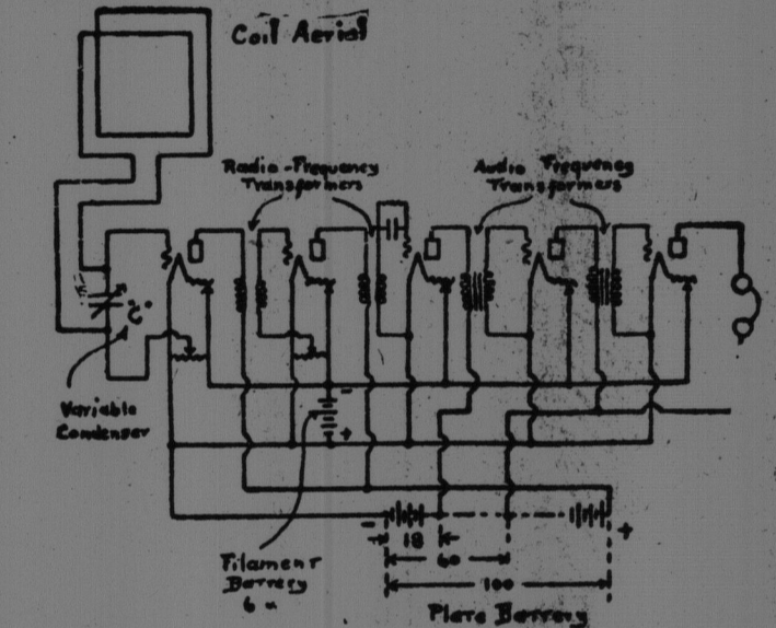
Amplifier - 2 Stages Radio - Detector - 2 Stages Audio.
