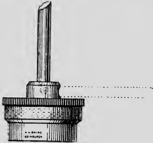
FIG. 8.—RADIUM APPLICATOR.
