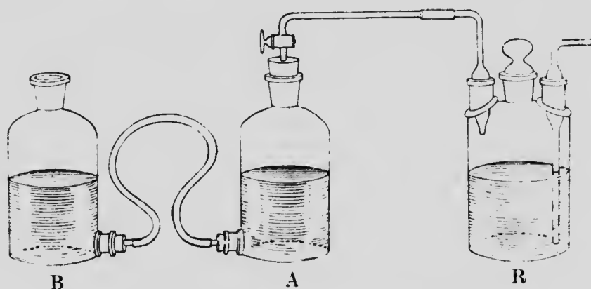
FIG. 11.—SIMPLE EMANATION APPARATUS.
