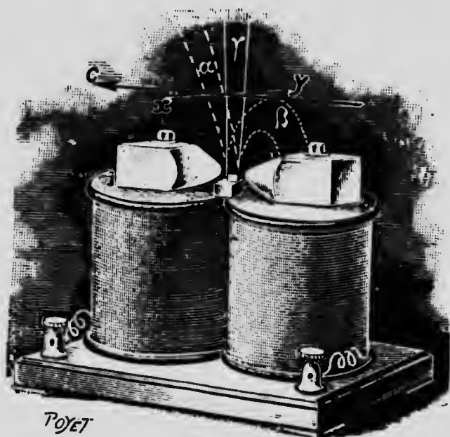
FIG. 5.—MAGNETIC DEFLECTION.
