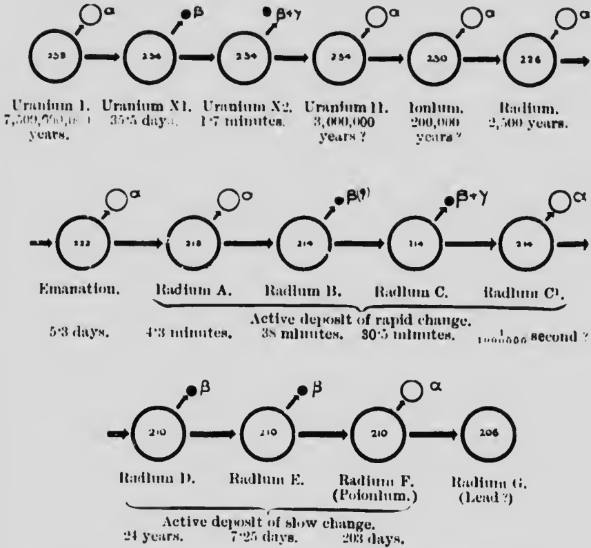
FIG. 7.—DISINTEGRATION SERIES (PROFESSOR SODDY).
