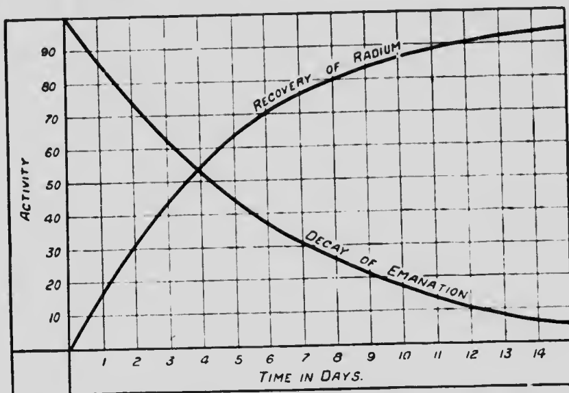
FIG. 6.—CURVE OF DECAY OF EMANATION AND OF RECOVERY OF RADIUM.
