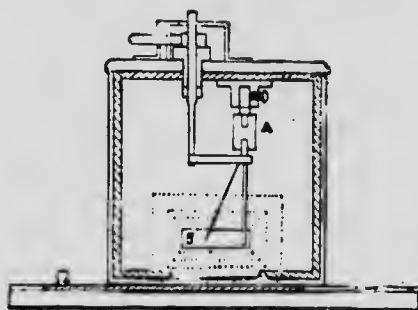
FIG. 9.—GAMMA-RAY ELECTROSCOPE.
