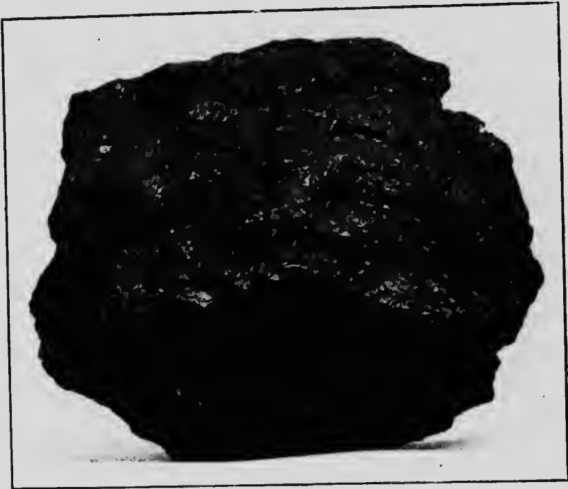
FIG. 4.—PITCHBLENDE.
