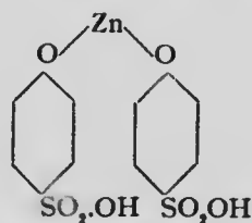
Zinc sulphocarbolate.
