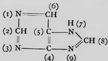
Purine.
