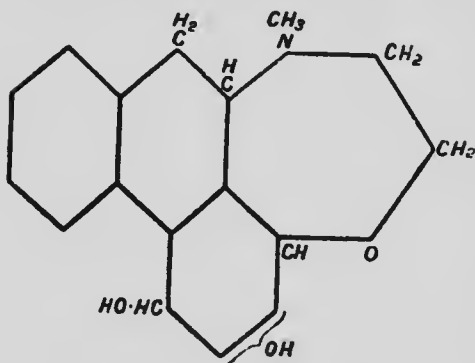
Knorr's Formula for Morphine.*
