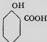
Salicylic acid.
