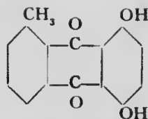
Chrysophanic acid (probable formula).
