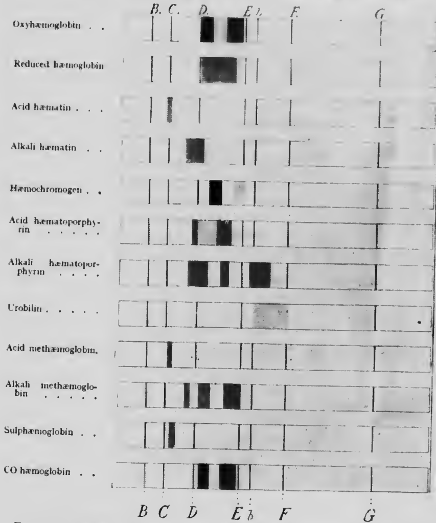
FIG. 68.—ABSORPTION SPECTRA OF HÆMOGLOBIN AND ITS DERIVATIVES.
