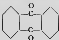
Anthraquinone.
