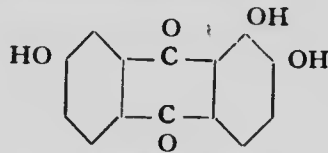
Anthrapurpurin. Purgatin is the diacetate.
