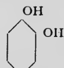
Pyrocatechin.
