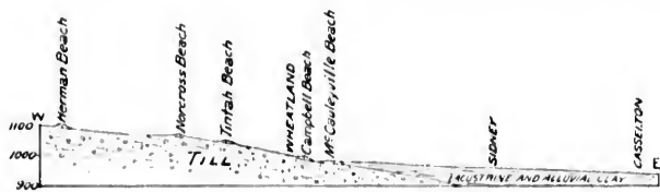
FIG. 23. Profile across beaches at and near Wheatland, N. Dak. Horizontal scale, 2½ miles to an inch.
