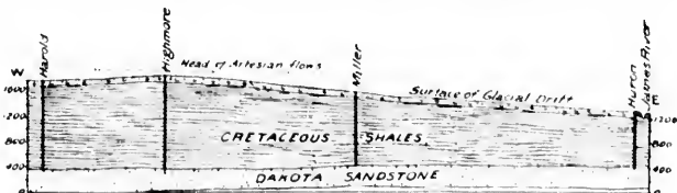
FIG. 35.—Section showing the series of artesian wells from Harold eastward to Huron. Horizontal scale, 45 miles to an inch.
