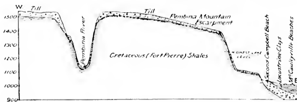
FIG. 28. Section on the international boundary, south of ranges 63 and 5, Manitoba. Horizontal scale, 25 miles to an inch.
