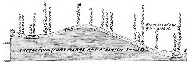
FIG. 8. Section across the Coteau des Prairies in Yellow Medicine County, Minn., and Deuel and Collington counties, S. Dak. Horizontal scale, 12 miles to an inch; vertical scale, 1,000 feet to an inch.
