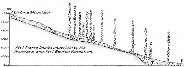
FIG. 29.—Section across ranges 6 and 5, Manitoba, 9 to 10 miles north of the international boundary. Horizontal scale, 24 miles to an inch.
