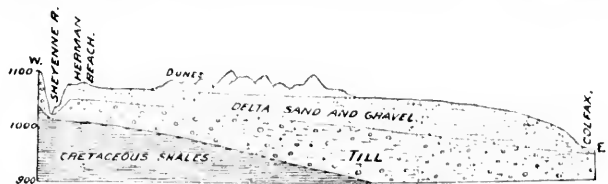
FIG. 13. Section across the delta of the Shyenne River. Horizontal scale, fowles to an inch.
