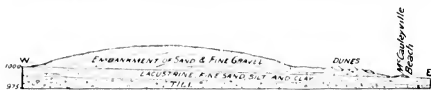
FIG. 19. Section across the Campbell embankment in sections 20 and 21, township 191, range 55. Horizontal scale, one third of a mile to an inch; vertical scale, 100 feet to an inch.
