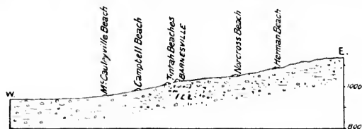
FIG. 20.—Profile across beaches at and near Barnesville, Minn. Horizontal scale, 2½ miles to an inch.
