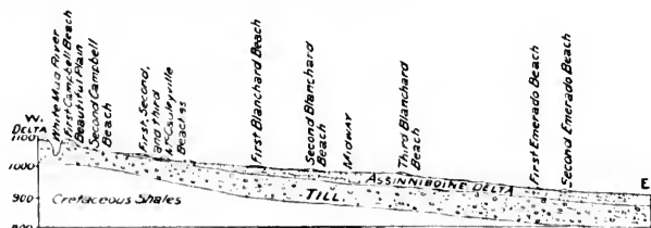
Fig. 30. Section on the south side of townships 15, ranges 13 and 12, Manitoba, between Arden and Gladstone. (Horizontal scale, 20 miles to an inch.)
