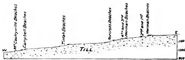
FIG. 22.—Profile across beaches on the north line of Onstead and Gaultrey, Minn., west of Maple Lake. Horizontal scale: 2 1/2 miles to an inch.
