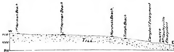
FIG. 24. Profile across beaches at Hunter, N. Dak., and westward. Horizontal scale, 2½ miles to an inch.
