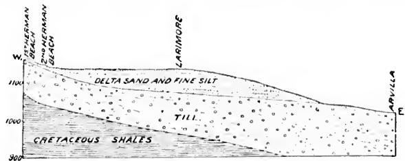
FIG. 11. Section across the delta of the Elk Valley. Horizontal scale 3 miles to an inch.
