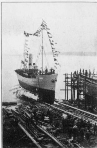
One of the Eight Trawlers built by the Davie Shipbuilding and Repairing Co. Limited
