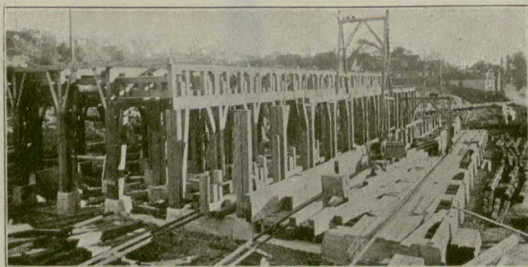
NO. 2.—SHOWS TRAVELLING CRANES AND METHOD OF ERECTING TRUSSES.
