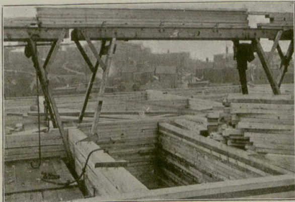
No. 5.—(A) Wedge Brackets. (B) Wedge Brackets in Service Supporting Platforms. (C) Movable Platforms. (D) Lumber Slides in Position. (E) Rolls.
