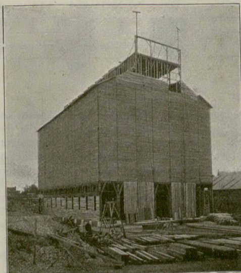
NO. 4.—ILLUSTRATING SUB-TIMBERING, PLANK MID-STRUCTURE, AND TIMBERING OF SUPERSTRUCTURE.
