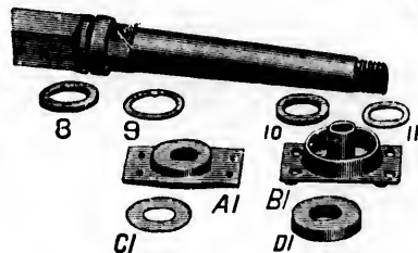
Patent Washers and Whiffletree Plate.
