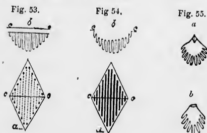
Fig. 53 Hydrospire of Caryoceras ornatus . a , surface view, the dots around the margin are the spiracles, the small dotted lines represent the course of the flat internal canals c, c , suture between the two plates; b , transverse section. Fig. 54. Hydrospire of Pleurocystites . a , surface view; c, c , suture; b , transverse section. Fig. 55 a . The same with the points c, c , drawn together; b , internal gill of a spider.
