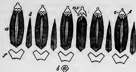
Fig. 73 Apex of Nucleocerinus Verneuilii Troost. g , ambulacral groove; p , pore through which groove enters into the interior; s , one of the ten spiracles; mv , oro-anal aperture. 74 Anterior side of a specimen; a , the anterior interradial. 75 Apex of a specimen which has lost the integument that covered the centre. 76 Diagram of the plates of the test; a , ambulacral plates; b , the basals; c , plates of the apex; d , one of the interradials; f , forked plate.
