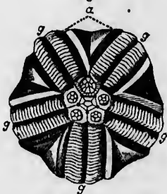
Fig. 60.—Diagrams of one pair of the hydrospires of a Pentremite ,— a , the inner side; b , the outer, or side attached to the shell; f , the fissure. 61. Section across an ambulacrum of a specimen of P. Godoni , enlarged 3 diameters.— l , lancelet plate; g , ambulacral groove; p , p , pores leading into the hydrospires; h , h , the two hydrospires, in transverse section. 62. Ideal figures of a transverse section through an entire specimen showing the ten hydrospires,— l , one of the five lancelet plates; p , p , pores; r , r , the two branches of one of the radial plates. 63. Summit of P. conoideus ,— a , anterior side; g , ambulacral grooves (copied from Dr. Shumard, but with the ovarian pores added).
