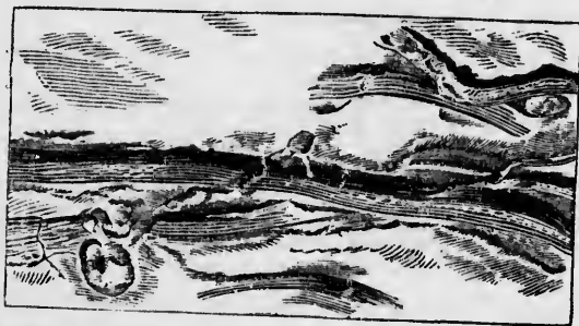
Fig. 32.— Eophyton Linnæanum? Torell. Part of a slab or sandstone with several fragments supposed to be of this species.
