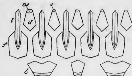
Fig. 71.—Calyceine plates of Pentramites ,— b , the basals; f , one of the five forked plates; d , deltoid plate; l , lancet plate; os , oral spiracle; s , spiracle.
