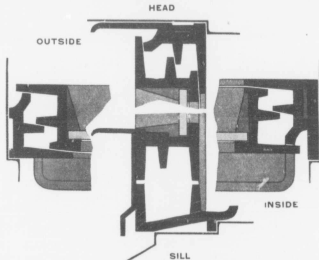
DETAILS HALF SIZE
