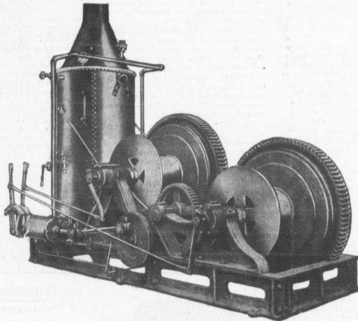
SPECIAL COMPOUND HAULAGE ENGINE.
