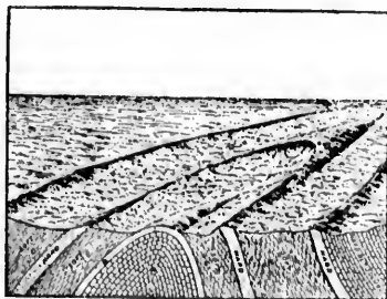
Anticlinal Fold, with Hemi-Cigar-Shaped Mountain.
