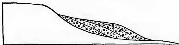
FIG. 14. Ideal Cross-Section of a Current-Built Terrace.
