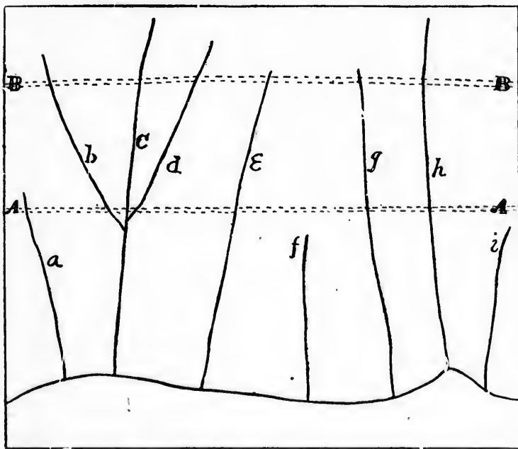
FIG. 16. Ideal Sketch-Map Showing Young Consequent Streams.
