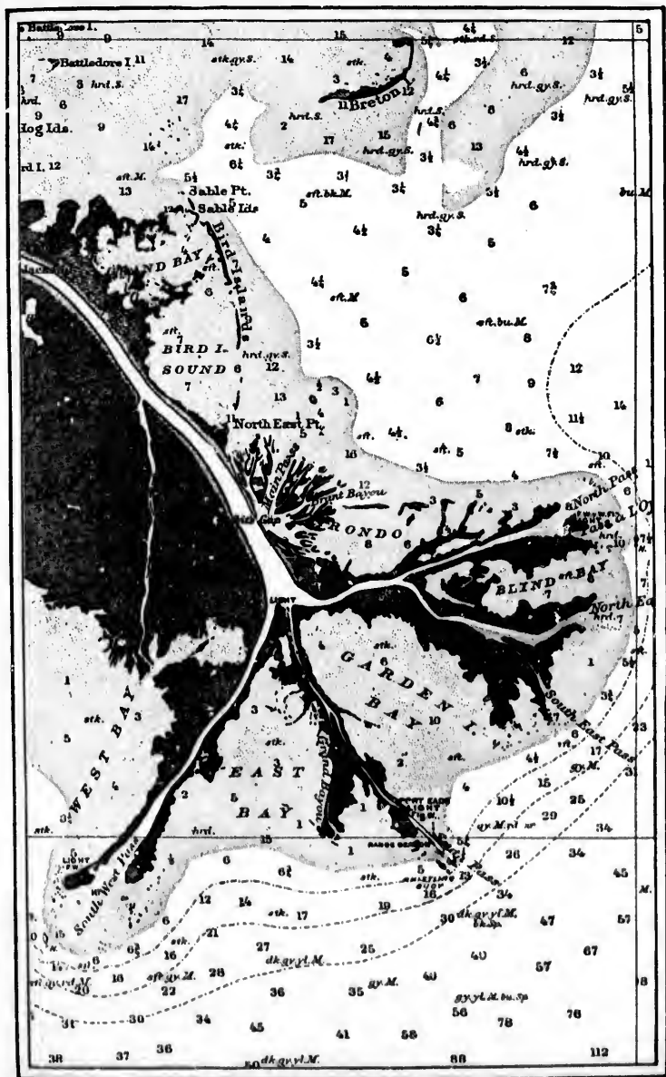
Delta of the Mississippi; by U. S. Coast Survey. Soundings on dotted areas in feet, all others in fathoms.
