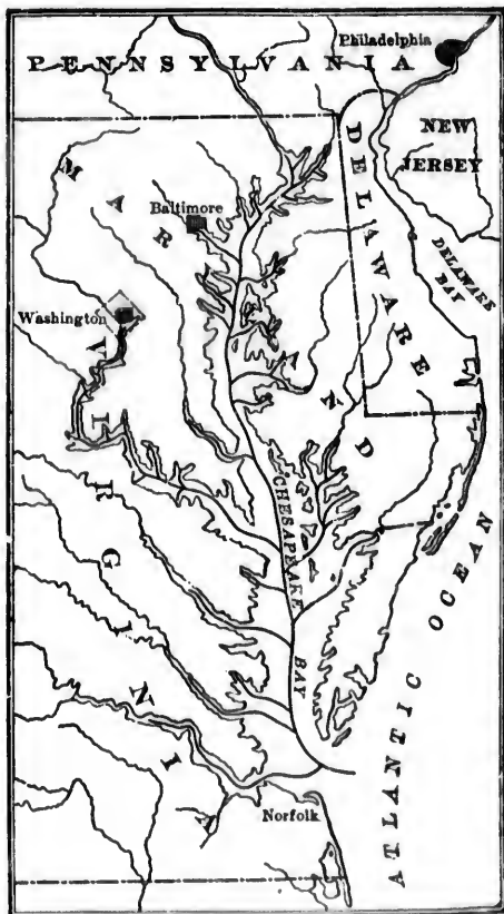
FIG. 22.—Map of Chesapeake Bay, Showing by Heavy Lines the Way in which Various Streams would Unite to Form a Single Trunk-Stream if the Land were Elevated. (After R. S. Tarr.)
