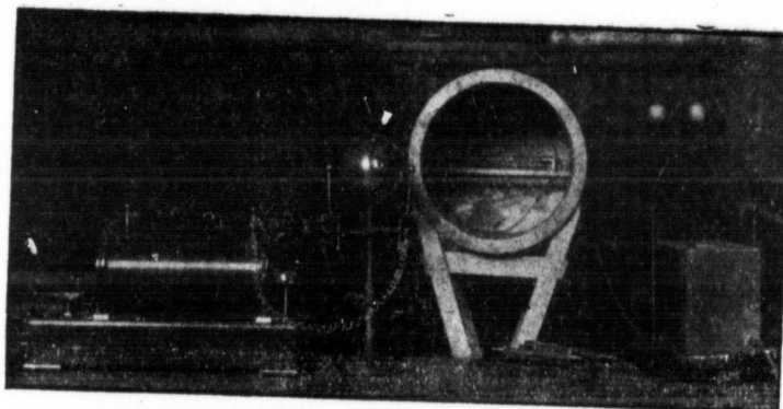
Fig. 9.—Actual apparatus used. Radiator connected to induction coil. Tube of turnings at back of copper hat, from which the covered wires lead to the galvanometer on the right. Two additional tubes on the table.
