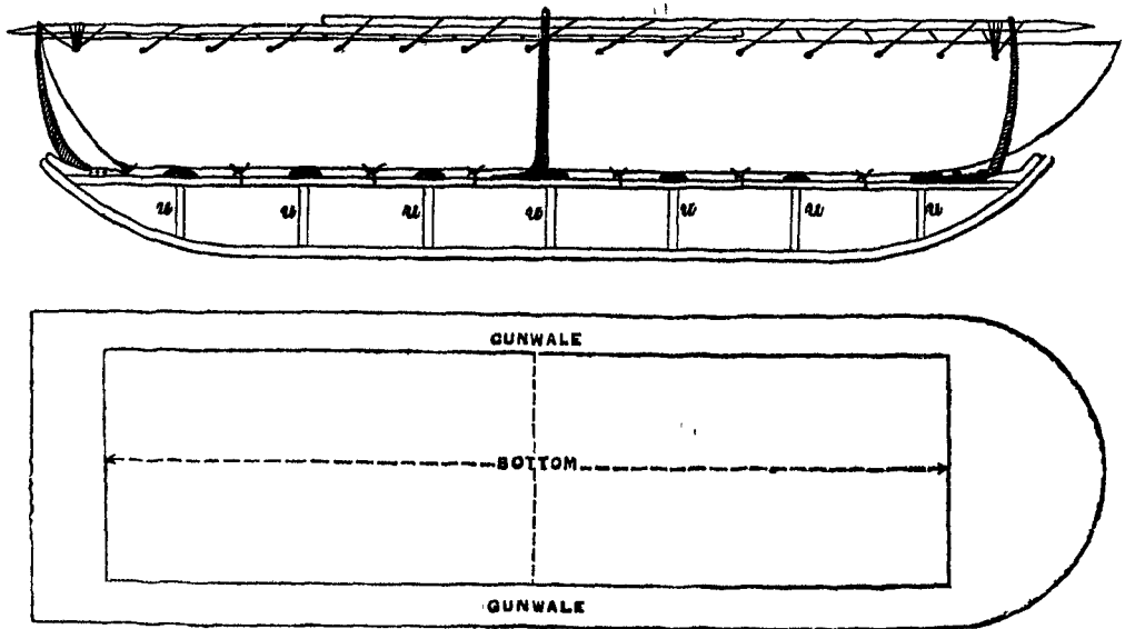
A broadside view of Sledge and Boat.
