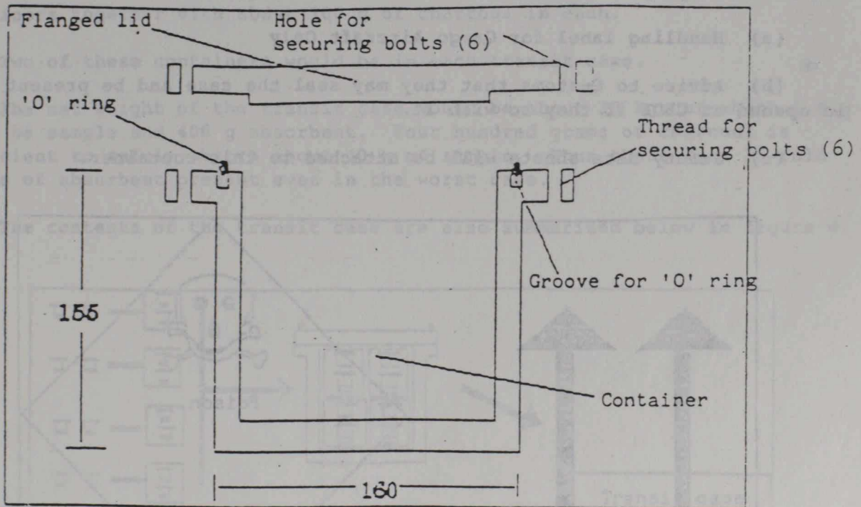
Figure 2: Schematic of tertiary container
