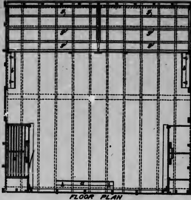
FLOOR PLAN
