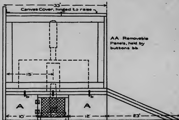
Fig. 2. Showing the end elevation of the brooder.
