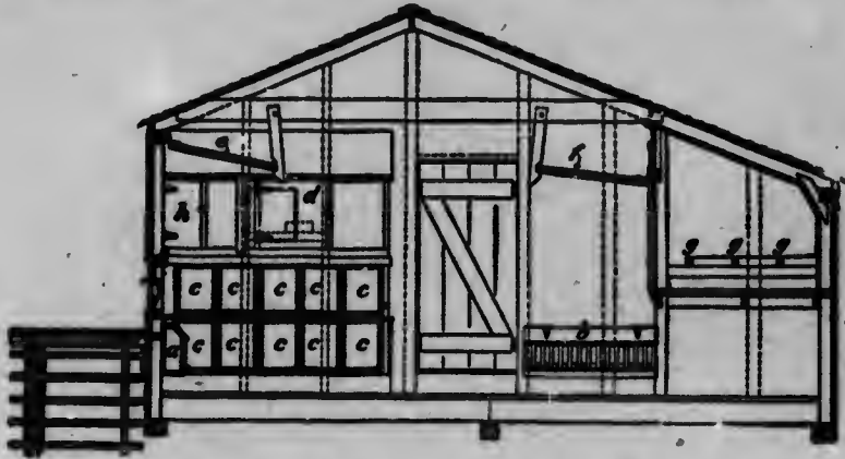
To show tie beams in combination-pitch house. b , feed-hopper; c , nests; d , coop for extra males; a , place for eggs; e , curtain; f , roost curtain (not needed); g , roosts.
