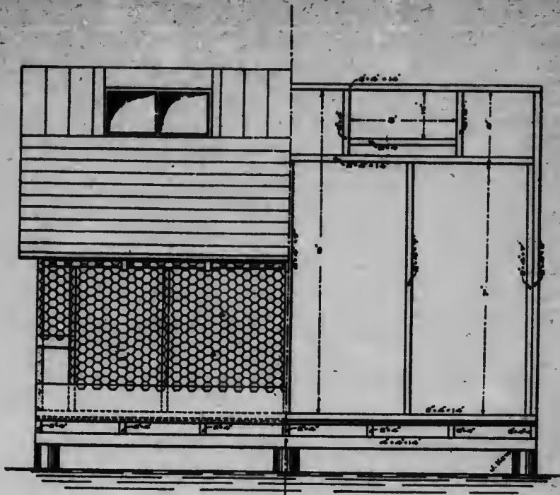
Front section cut through Woods house.
