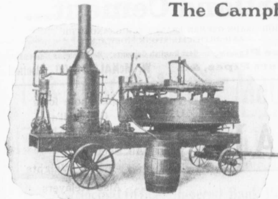
1/2 YARD SIZE MOUNTED ON TRUCKS.
