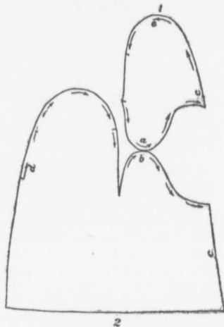
Figure 3. Pattern of sealskin mitten.
