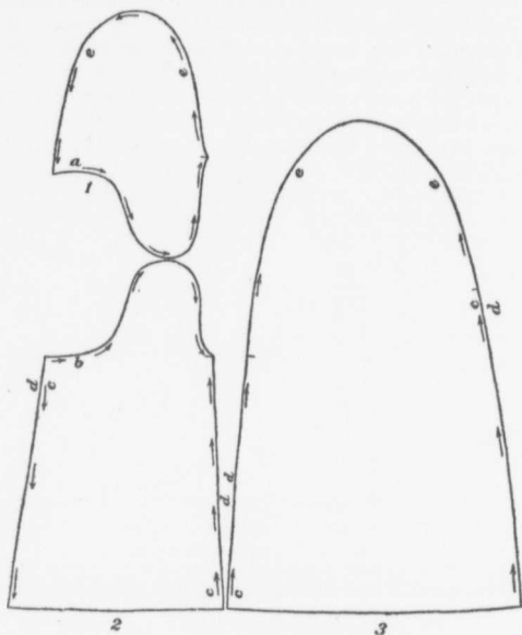
Figure 5. Pattern of waterproof mitten.
