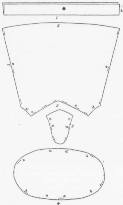
Figure 1. Pattern of waterproof skin boot.
