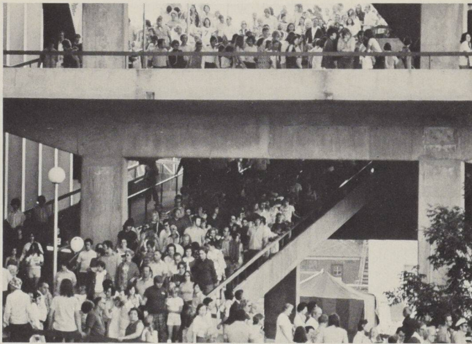
Ottawa's Lansdowne Park stadium has wide exterior ramps for egress rather than the interior stairs and escalators used in Calgary.
