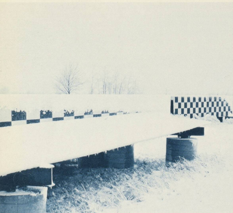
Snow accumulation studies on the inverted 'T' monorail track configuration show its unsuitability for Canadian conditions.
