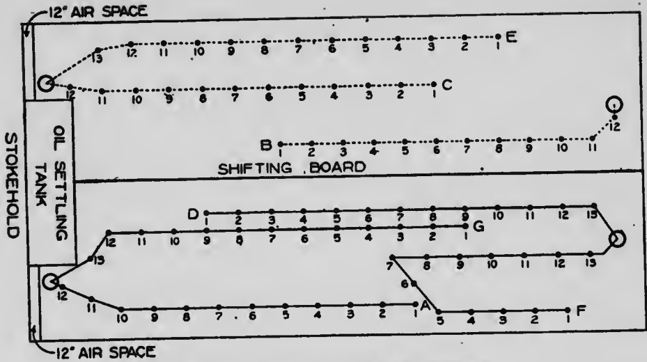
Fig. 9. Plan of forward hold showing thermometers.
