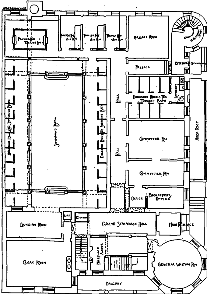
PLAN OF PROPOSED ATHLETIC CLUB BUILDING, TORONTO.
