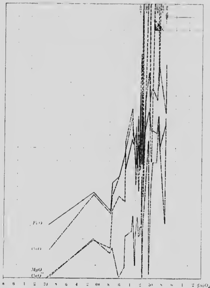
FIG. 6. Molecular proportions of magnesia, lime and iron oxide in banakites, -hoshonites and absarokites, Yellowstone National Park.
