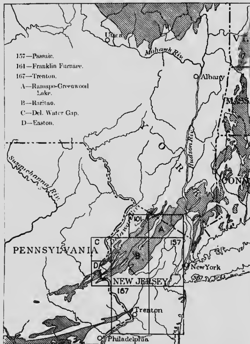
FIG. 1.—Sketch map showing areas of Pre-Cambrian crystalline rocks (shaded) in New Jersey and adjacent states, with the names of the quadrangles in New Jersey upon which folios have been published, or are in course of publication, by the U. S. Geological Survey. The names preceded by figures are of folios that have been published.
