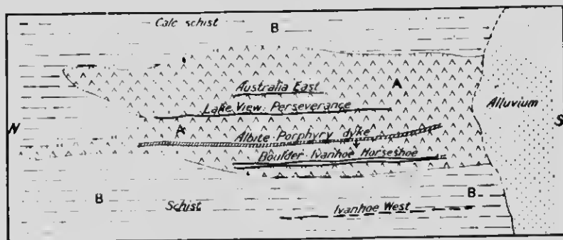
FIG. 1. Diagrammatic plan of productive area of Kalgoorlie, Western Australia, showing principal lode-channels.
