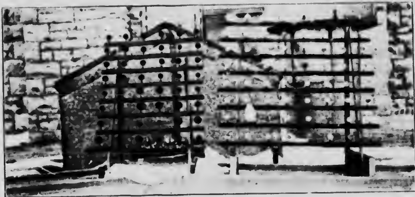
Corrosion tests: method of exposing alloy discs.
