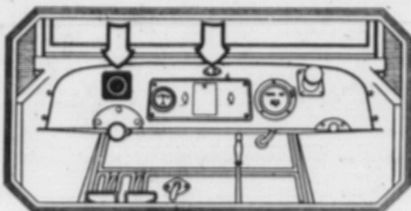
Dashboard board, showing gasoline gauge and electric dash light, as well as speedometer, electric starting and lighting plugs and ammeter. See arrows.
