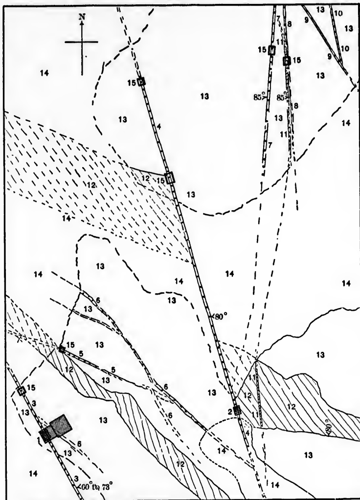
Group of Veins, Sirdar Gold Mine, Scale 1650, linear, to 1.
