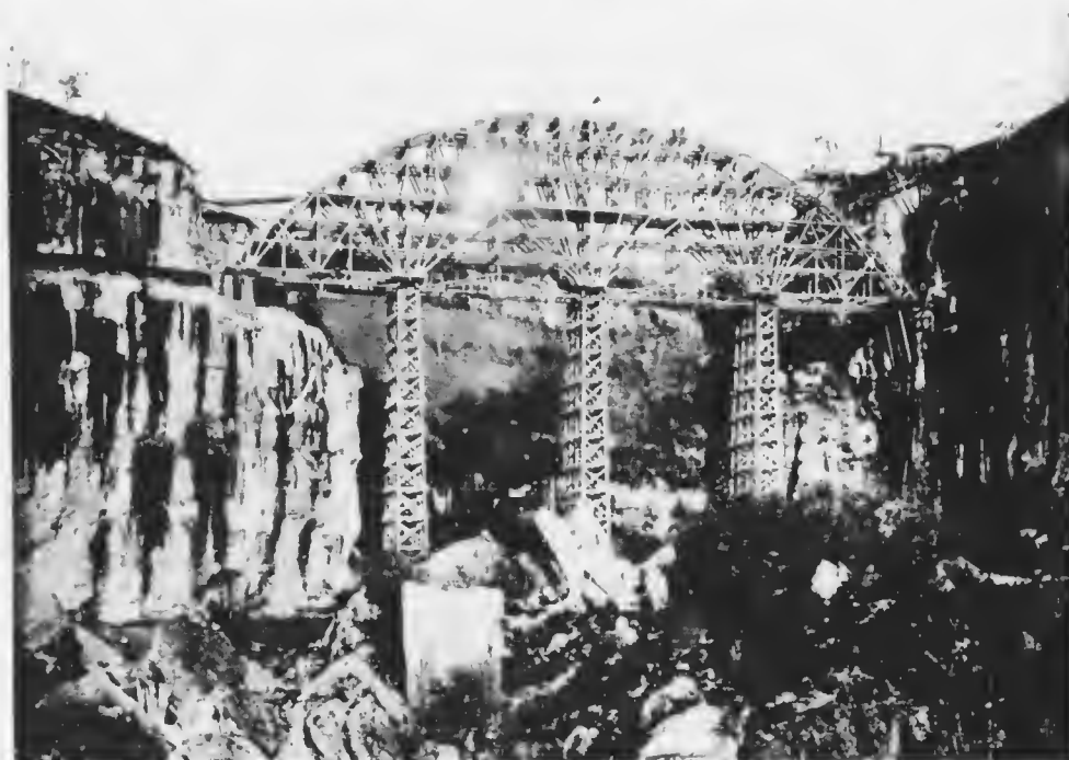
THE MONTANGAS BRIDGE IN COURSE OF CONSTRUCTION
