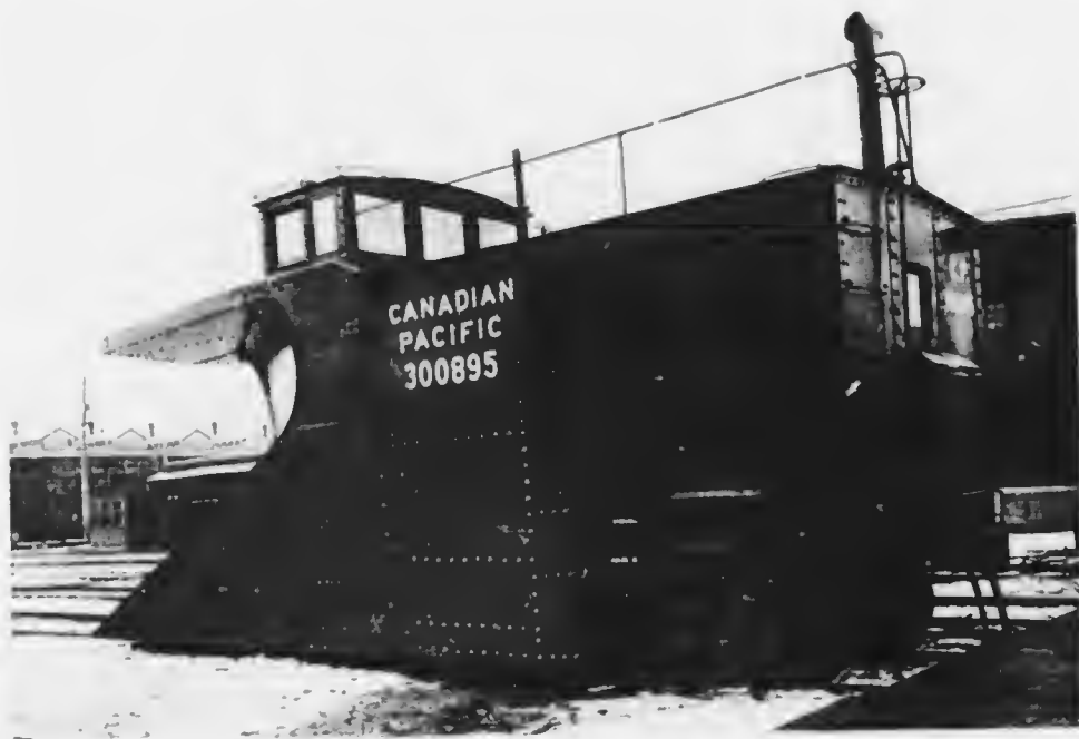
GENERAL VIEW OF THE CANADIAN PACIFIC WEDGE SNOW-POUGH.
