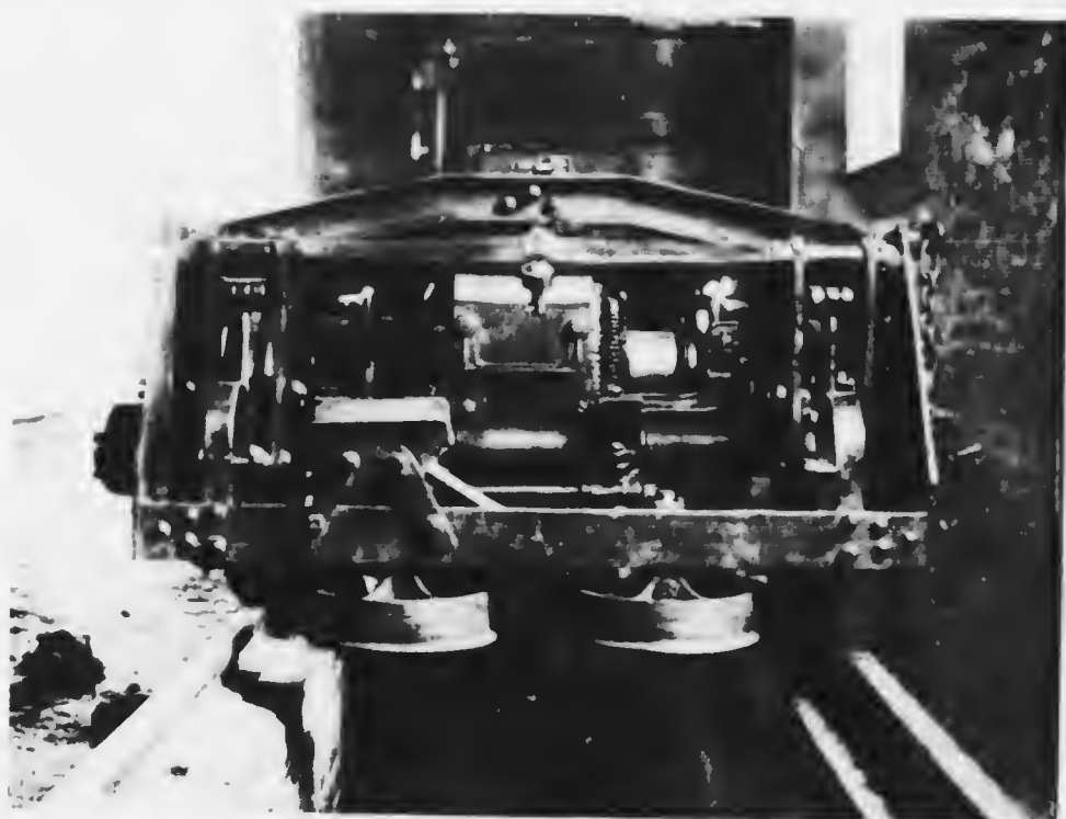
UNDERNEATH VIEW OF THE FELL ENGINE. Showing the horizontal wheels which grip the centre-rail.
