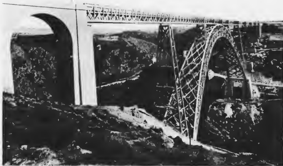
THE GABARIT VIADUCT ACROSS THE TRUEYRE GORGE. Designed by M. Eiffel, this bridge is 400 feet above the floor of the rift. The span is 541 feet.
