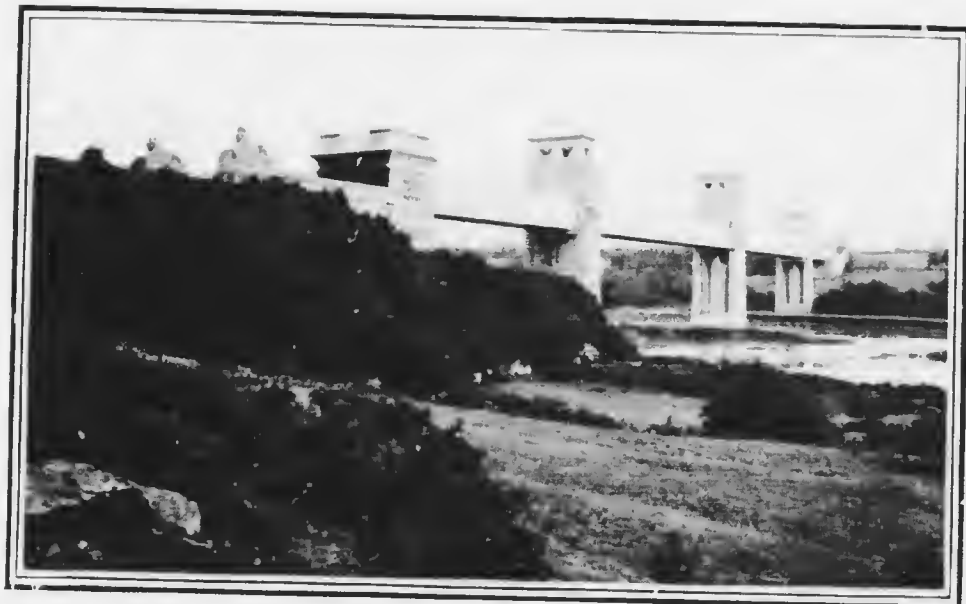
THE TUBULAR BRIDGE, DESIGNED BY STEPHENSON, OVER THE MENAI STRAITS.
