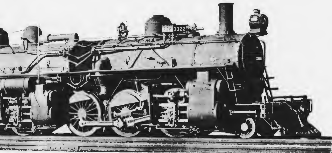
BUILT FOR FREIGHT SERVICE UPON THE ATCHISON, TOPEKA AND SANTA FE RAILWAY. The front part carries the feed-water heater tubes. In running order the complete locomotive weighs 278½ tons.
