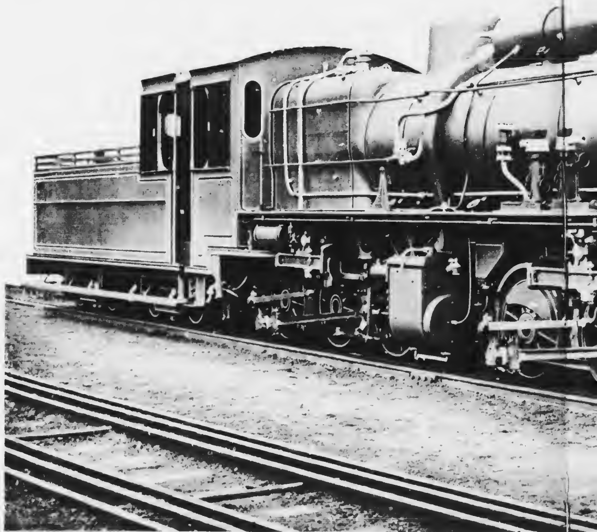
THE HEAVY 0-6-6-0 BRITISH-BUILT COMPOUND
