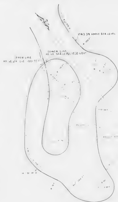
LOOP NO. 2 AT 14th MILE. GRADIENT 1 IN 28.
