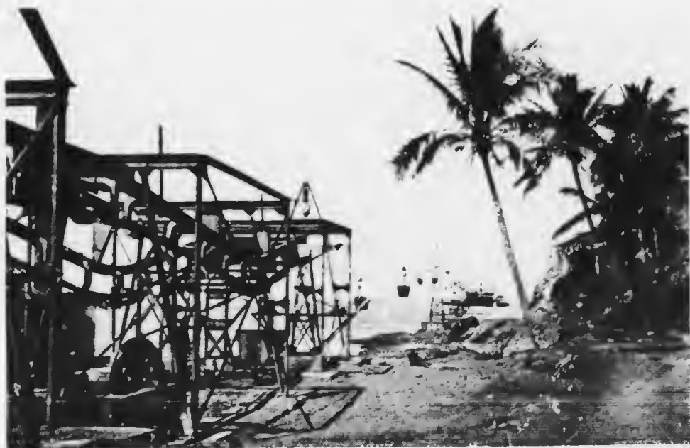
THE NICKEL ORE AERIAL RAILWAY IN NEW CALEDONIA.
