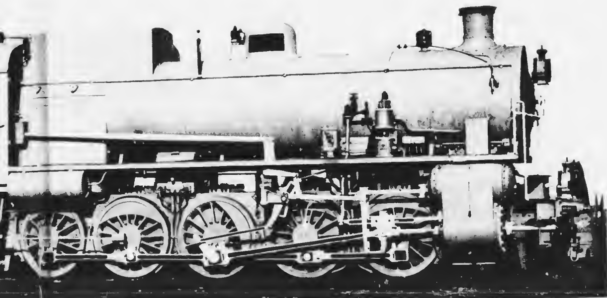
FOUND tinuous he coal LOCOMOTIVE USED ON THE ITALIAN STATE RAILWAYS grades of 1 in 38.4 and 1 in 40 are encountered. The tender, carrying water only, and a brake compartment, banker of 4 tons capacity is mounted on top of the boiler forward of the cab.
