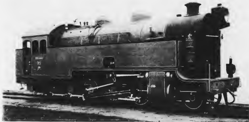
POWERFUL TEN-WHEEL-COUPLED SUPERHEATED LOCOMOTIVE ENGAGED IN SAND HAULAGE IN UPPER SILESIA
