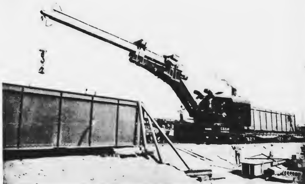
AN INDUSTRIAL WORKS WRECKING CRANE ADAPTED TO HANDLE AN AWKWARD LOAD. An extemporised boom attached to the crane-jib enabled this machine to place unaided an 80-foot girder weighing 20 tons.
