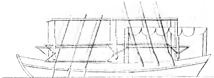
PLAN OF THE HULL OF A STEAMER OF 100 TONS
